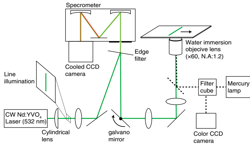
Fig. S1. Optical setup for a slit-scanning Raman microscope.
