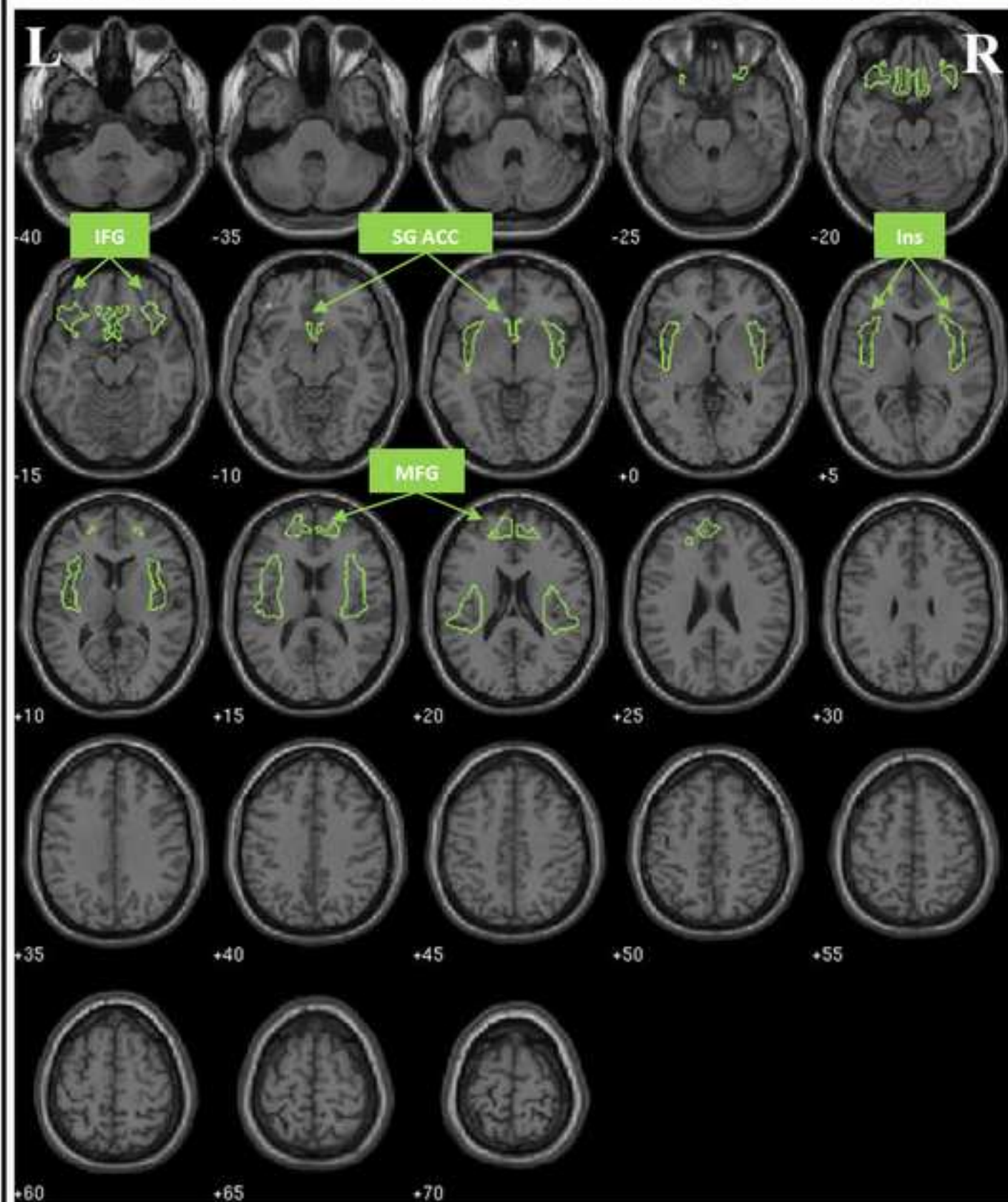
FIGURE S1. REGIONS OF INTEREST FOR EVALUATIVE AFFECTIVE CIRCUIT
