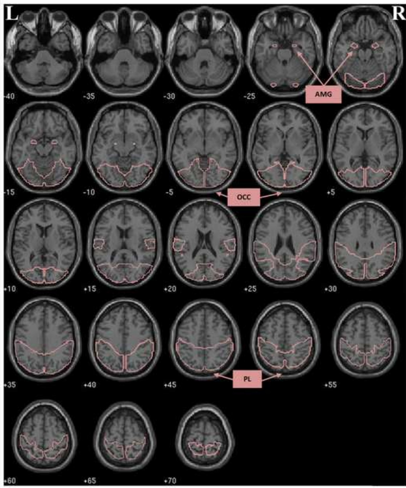
FIGURE S2. REGIONS OF INTEREST FOR REACTIVE AFFECTIVE CIRCUIT
