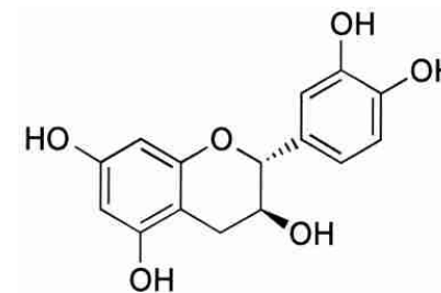
Catechin
