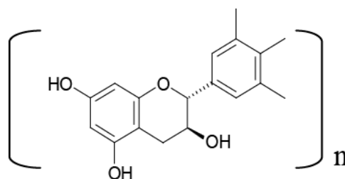
Proanthocyanin
