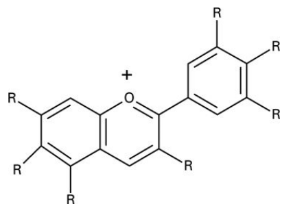
Anthocyanin
