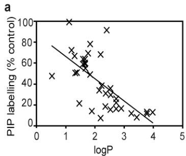
Fig. S1. Comparison of lipophilicity (logP) values with PIP labelling show increased phosphoinositide attenuation with lipophilicity ( P < 0.001 ) for novel VPA-related compounds.
