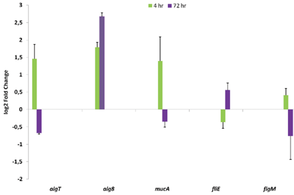
Figure 1. qRT-PCR quantification of selected transcripts in KT2440 after 4 and 72 hr matrix stress
