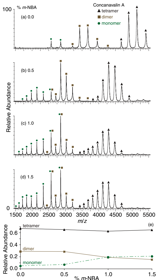
Figure 1. Nanoelectrospray mass spectra of \sim 10 \mu\text{M} concanavalin A in 200 mM ammonium acetate, pH 6.8, aqueous solution containing (a) 0%, (b) 0.5%, (c) 1.0%, and (d) 1.5% m -NBA. The normalized abundances of concanavalin A monomer, dimer, and tetramer as a function of m -NBA concentration are shown in (e)
