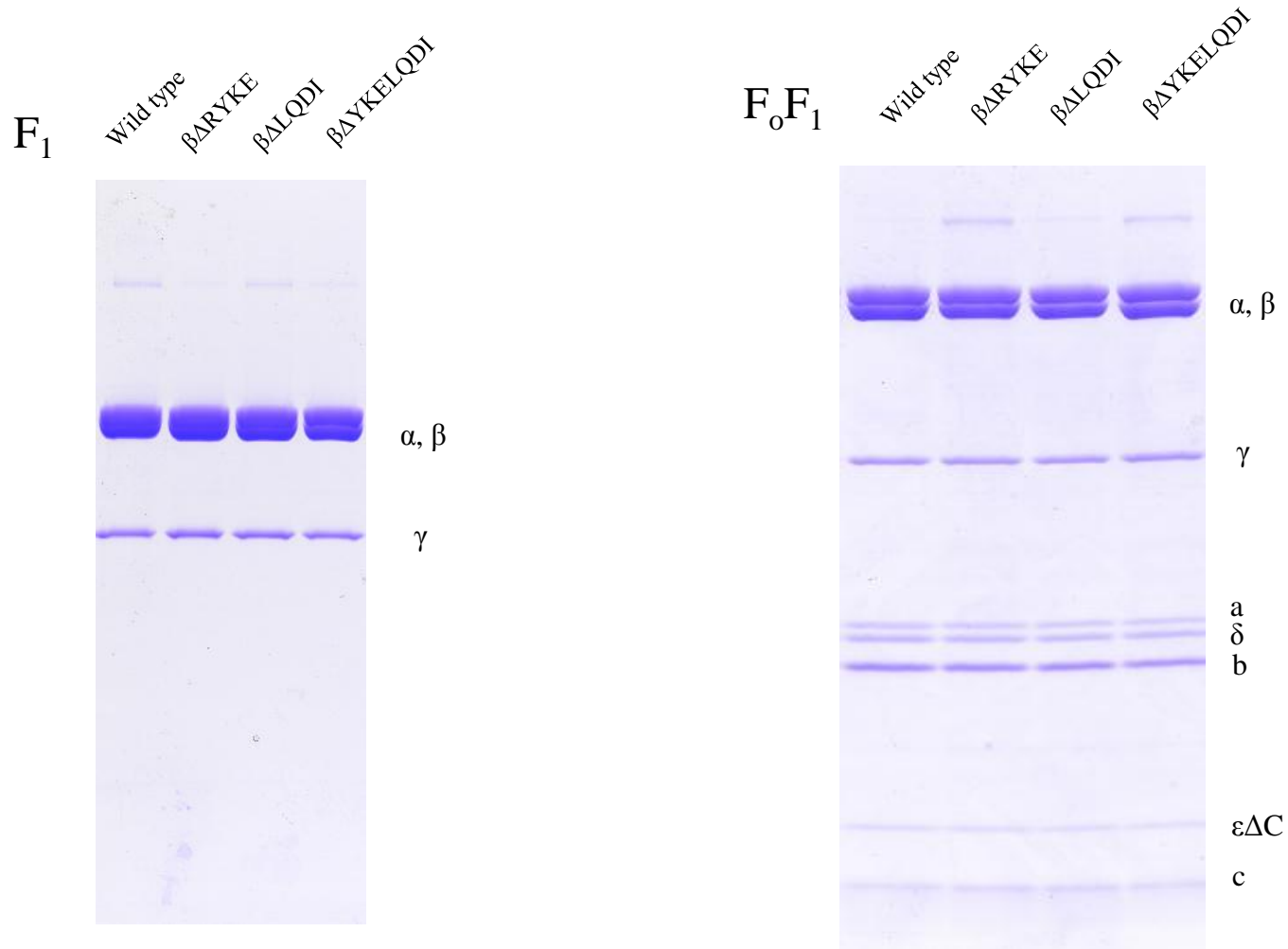
Fig. S1. Purity of the mutant enzymes used in this work
