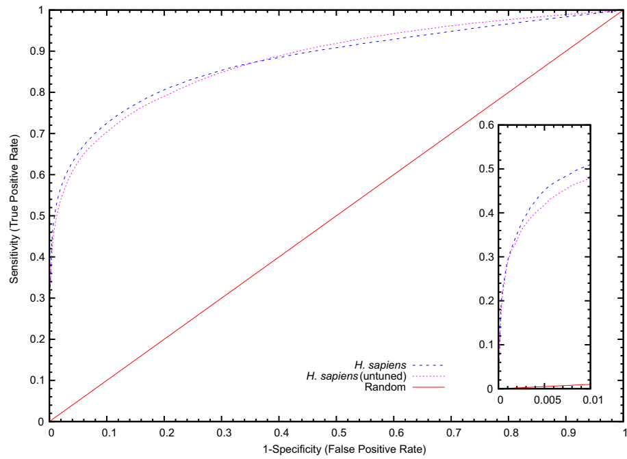
Figure S9. Difference between using tuned and untuned parameters to predict human PPIs. ROC curve presents the True Positive Rate (Sensitivity) against the False Positive Rate (1-Specificity). Inset: performance at very high specificity (99.95%).
