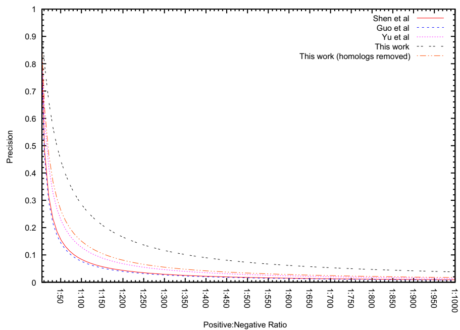
Figure S2. Comparison of precision over human proteins for competing methods. Precision for the current method (before and after the removal of homologs) is higher than those of competing methods for different positive: negative ratios. It should be noted that homologs are not removed in the competing methods.
