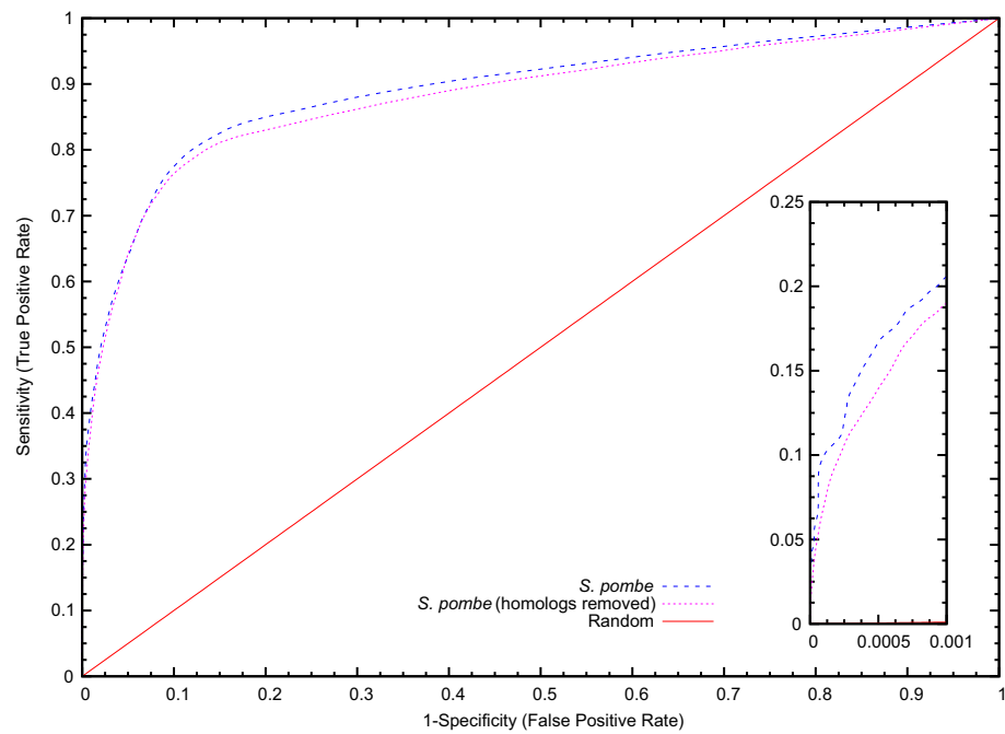
Figure S7. ROC curve with and without homologous sequences for S. pombe . The curve presents the True Positive Rate (Sensitivity) against the False Positive Rate (1-Specificity). Inset: performance at very high specificity (99.95%).
