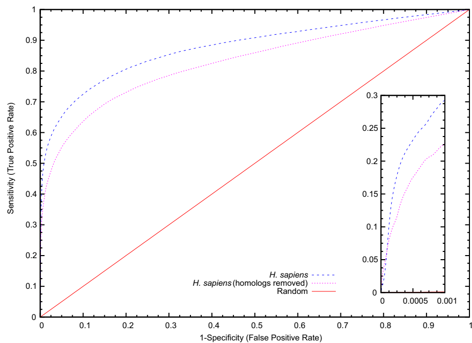
Figure S5. ROC curve with and without homologous sequences for human. The curve presents the True Positive Rate (Sensitivity) against the False Positive Rate (1-Specificity). Inset: performance at very high specificity (99.95%).
