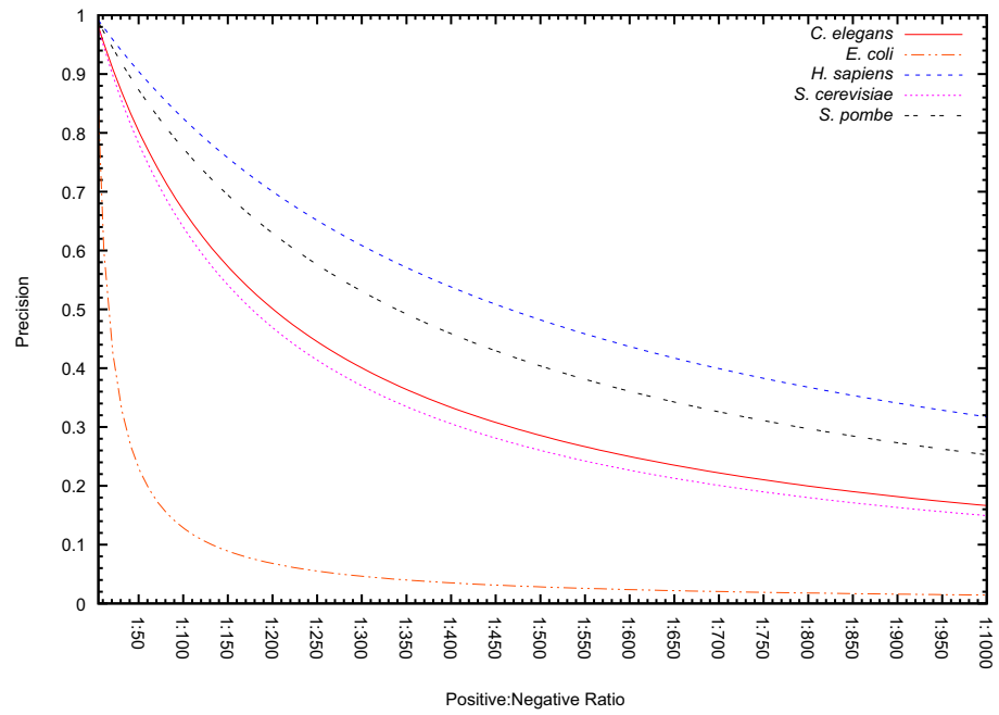
Figure S1. Impact of the positive: negative ratio on the precision. Precision is reduced as positive: negative ratio is reduced.
