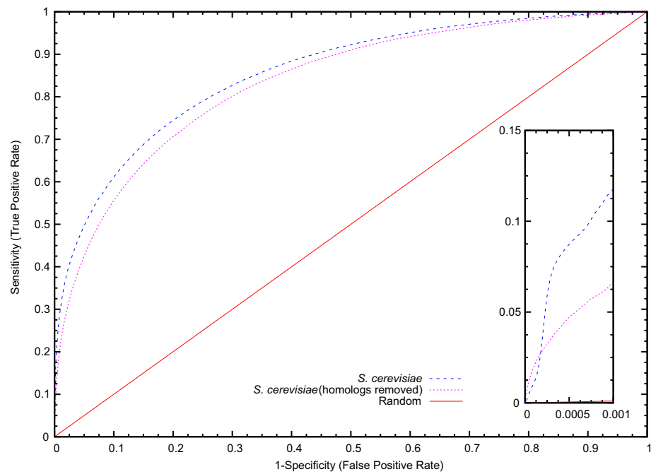
Figure S6. ROC curve with and without homologous sequences for S. cerevisiae . The curve presents the True Positive Rate (Sensitivity) against the False Positive Rate (1-Specificity). Inset: performance at very high specificity (99.95%).
