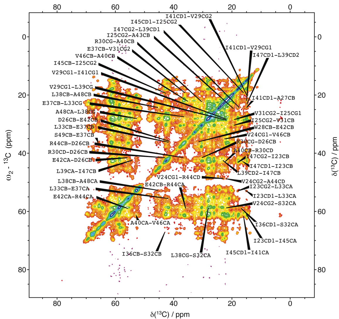
Figure S2. DARR spectrum with a 250 ms mixing period.
