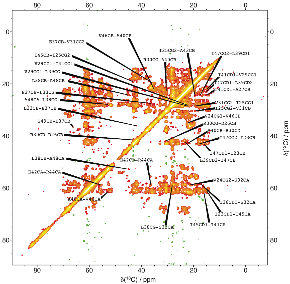
Figure S1. PAR spectrum with a 10 ms mixing period.
