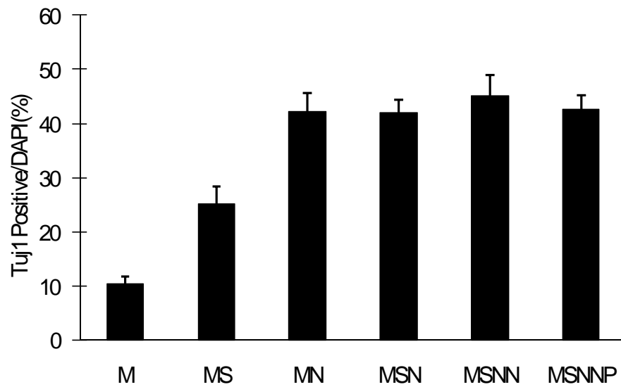
Figure S5. Fraction of surviving cells that stained positive for Tuj1 cell IMR90 cells transduced with various combinations of transcription factors. The error bars represent SEM, n=5. M: Mash1; MS: Mash1+Sox2; MN: Mash1+Ngn2; MSN: Mash1+Sox2+Ngn2; MSNN: Mash1+Sox2+Ngn2 +Nurr1; MSNNP: Mash1+ Sox2+Ngn2 +Nurr1+Pitx3.
