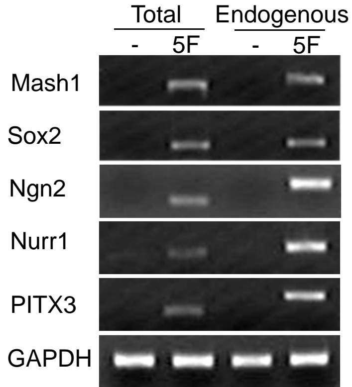
Figure S7. Semi-quantitative PCR analysis of the expression of five factors in parent IMR90 (as denoted by a “-” sign) as well 5F-transduced IMR90 cells. Total level indicates endogenous+exogenous expression while endogenous indicates expression from only the endogenous genes. The positions of the total and endogenous bands are different because different primers for total and endogenous PCR were used to distinguish the two. See Table S4 for specific primer sequences.
