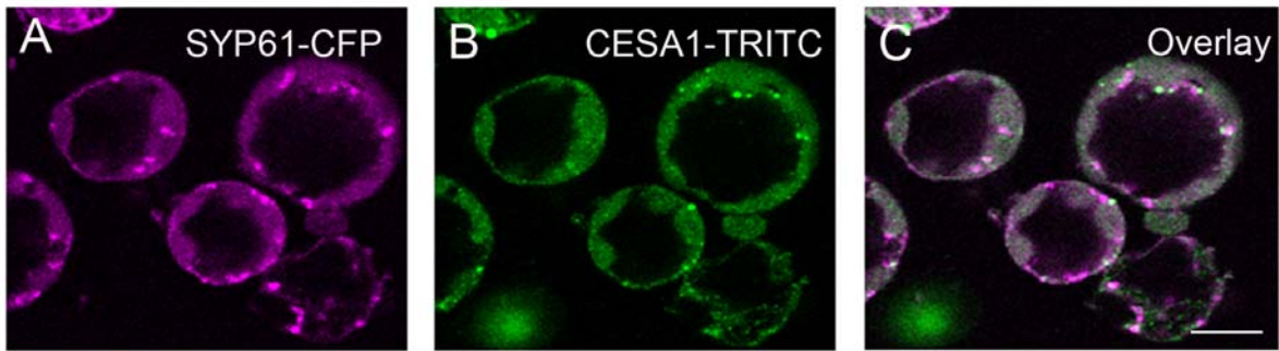
Supplementary information, Figure S5 Colocalization of SYP61 with CESA1 in Arabidopsis protoplasts.
