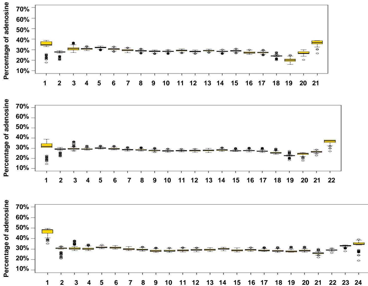
Supplemental Figure S4. Percentage of adenosine at each position of 21-nt, 22-nt, and 24-nt small RNAs of the 162 Arabidopsis small RNA deep sequencing data sets deposited in the NCBI GEO database.
