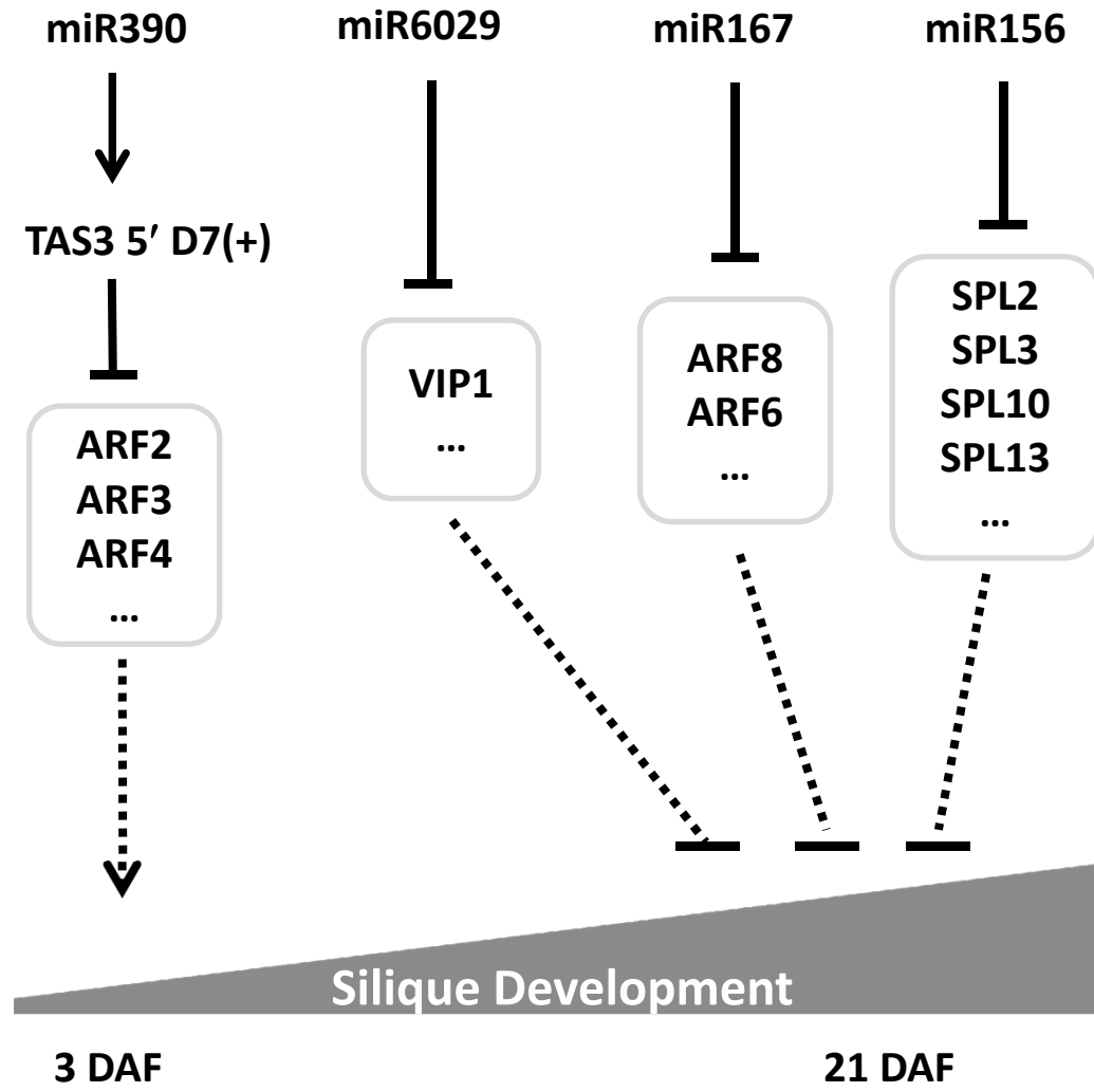
Supplemental Figure S7. A proposed model of the regulation of B.napus early silique development via miRNAs, ta-siRNA, and their target genes.
