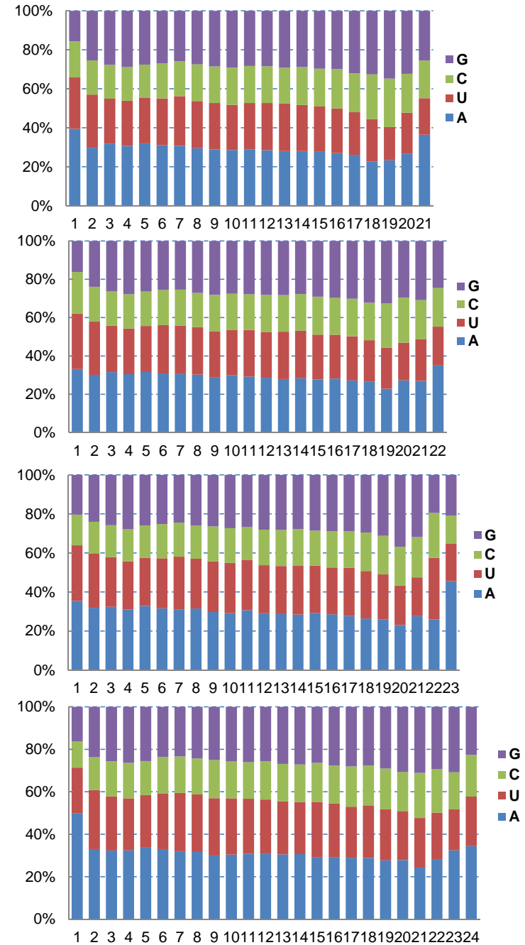
Supplemental Figure S2. Nucleotide preferences at each position of small RNAs. A, Nucleotide preferences of the total sequenced 21-nt, 22-nt, 23-nt, and 24-nt non-redundant sequences. B, Nucleotide preferences of the 21-nt, 22-nt, 23-nt, and 24-nt non-redundant sequences mapped to the Brassica BAC clones.
