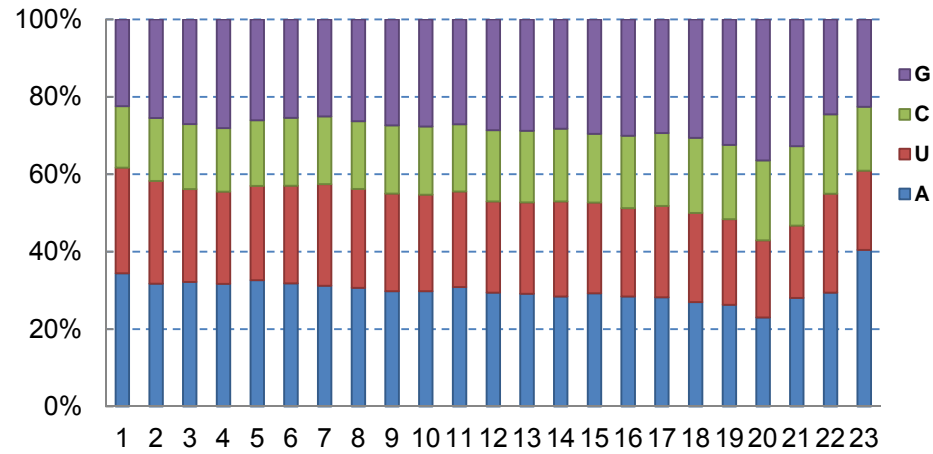
Supplemental Figure S3. Nucleotide preference at each position of the 24-nt dependent 23-nt small RNAs. A, Nucleotide preference of 23-nt small RNAs with identical 5' ends to the 24-nt ones. B, Nucleotide preference of 23-nt small RNAs with identical 3' ends to the 24-nt ones.
