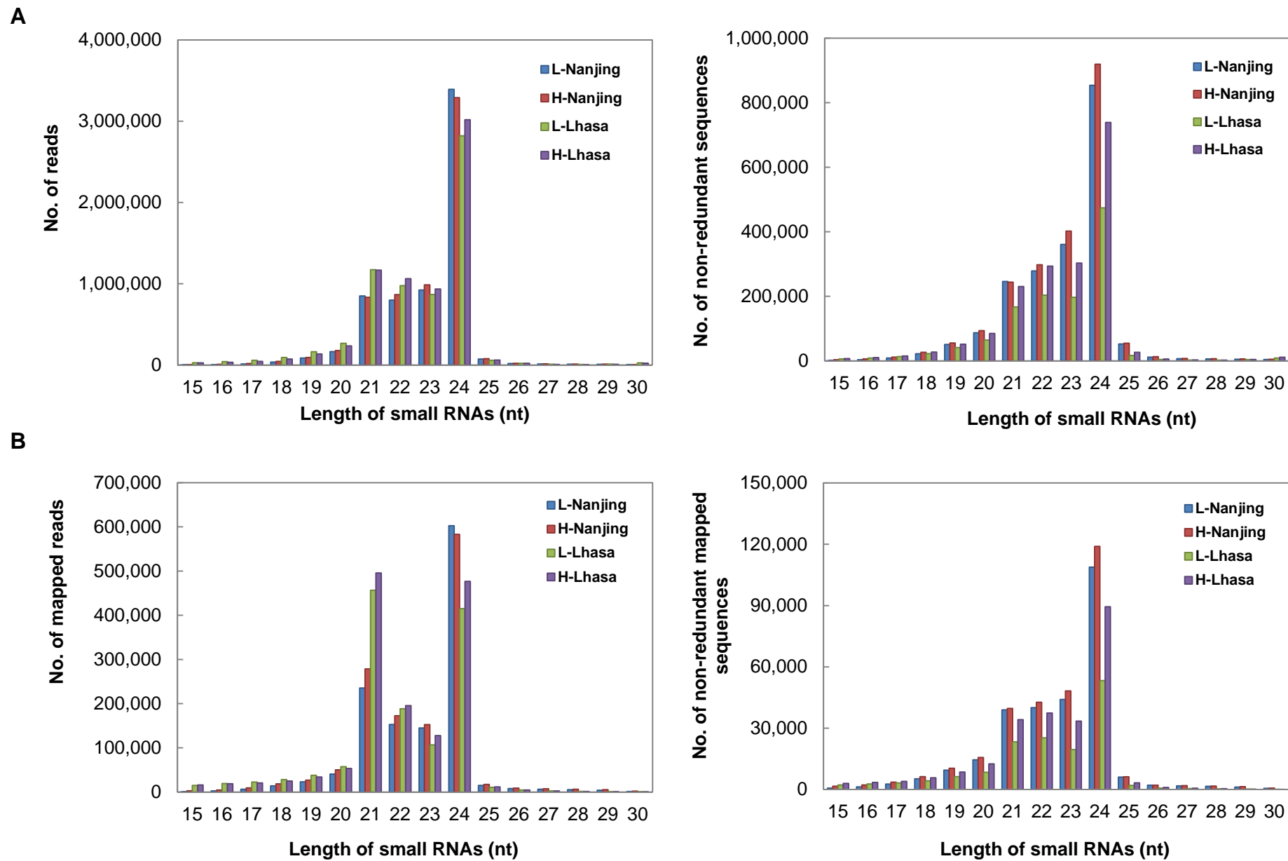
Supplemental Figure S1. Size distribution of small RNAs. A, Size distribution of total sequenced reads and non-redundant sequences; B, Size distribution of total sequenced reads and non-redundant sequences mapped to the Brassica BAC clones.
