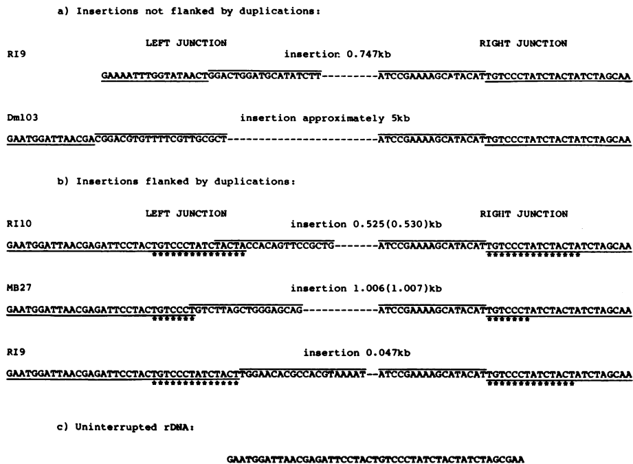
Figure 3. A Comparison of Insertion Junctions The rDNA sequences to the left and right of insertions are shown in alignment to facilitate comparison. The one exception is the sequence to the left of the 747 nucleotide insertion in RI9, where the rDNA originates from the 28S \beta 2 region rather than the 28S \beta 1 region as in the other cases (see also Fig. 1). This cloned segment is unusual in that it contains two insertions 380 nucleotides apart. Strictly speaking this insertion is flanked by a duplication of this 380 nucleotide sequence, but we have placed it in a separate category together with Dm103, since the structure of the clone is so unusual. The sequence at the left hand junction in Dm103 is from Roiha et al. (15). The rDNA sequences are underlined and the insertion sequences overlined. The duplicated sequence is indicated by the asterisks. The sequence of uninterrupted rDNA (15) is shown for comparison.
