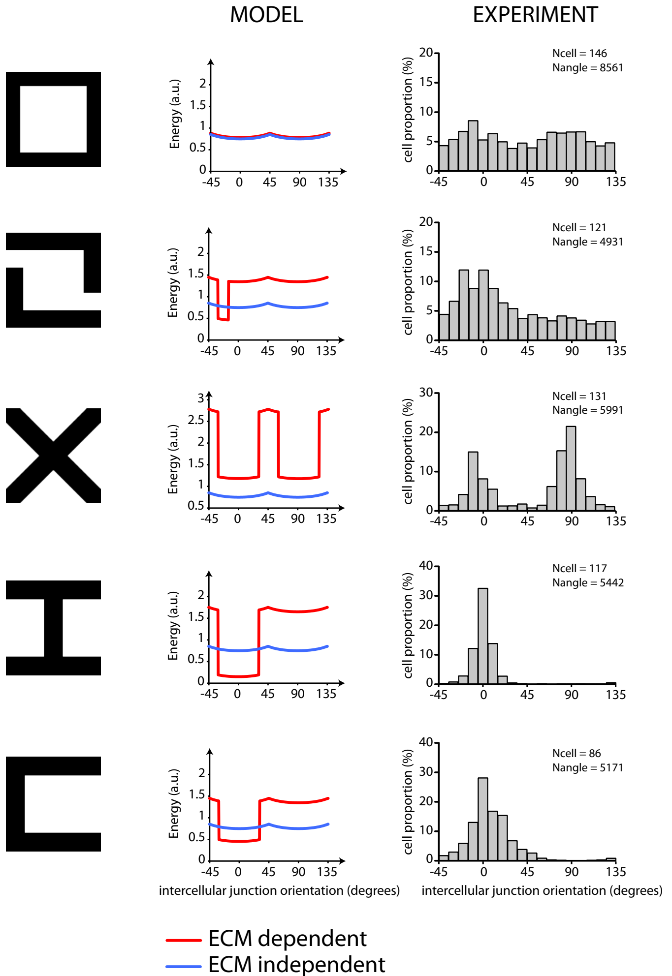
Figure S7: Modeling of the energetic cost of intercellular junction positioning
