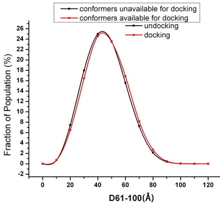
Figure S3-End-to-end distance distributions of D1-40 and D61-100 for the constructed 100mer peptide.
