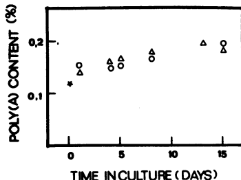
Fig. 1 - Poly(A) content of cytoplasmic RNA as a function of culture time.
