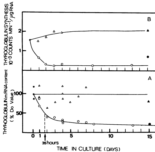
Fig. 5 - Tgb mRNA quantitation in cytoplasm of TSH-treated and control cells as a function of culture time.
