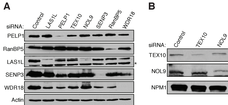
Figure S1. Antibodies used in this study are specific for the corresponding protein. (A) HEK 293T cells were transfected with the indicated gene-specific siRNA. After forty-eight hours, cells lysates were separated by SDS-PAGE and analyzed by Western blotting with the indicated antibody. (B) HEK 293T cells were transfected with the indicated gene-specific siRNA. After forty-eight hours, nucleolar extracts were separated by SDS-PAGE and analyzed by Western blotting with the indicated antibody.
