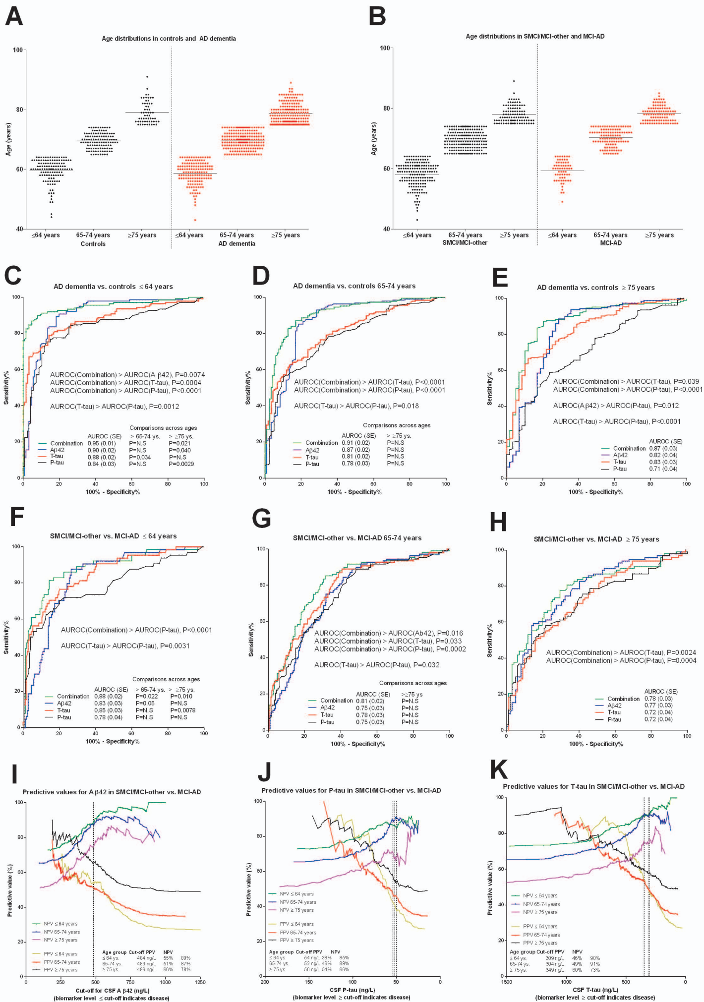
Figure e-1. Age level cut-distributions in controls and AD dementia (A), SMCI/MCI-other and MCI-AD (B). ROC curves for individual biomarkers and for a combination of biomarkers ("Combination") within age groups (panels C-H). Comparisons of AUROCs across age groups are shown in panels C-D and F-G. Predictive values across the entire ranges of possible cut-offs in MCI patients (panels I-K, the dotted lines indicate specific cut-offs generated at 85% sensitivity for AD dementia, data points with 95% confidence intervals ranging more than 50% are excluded).
