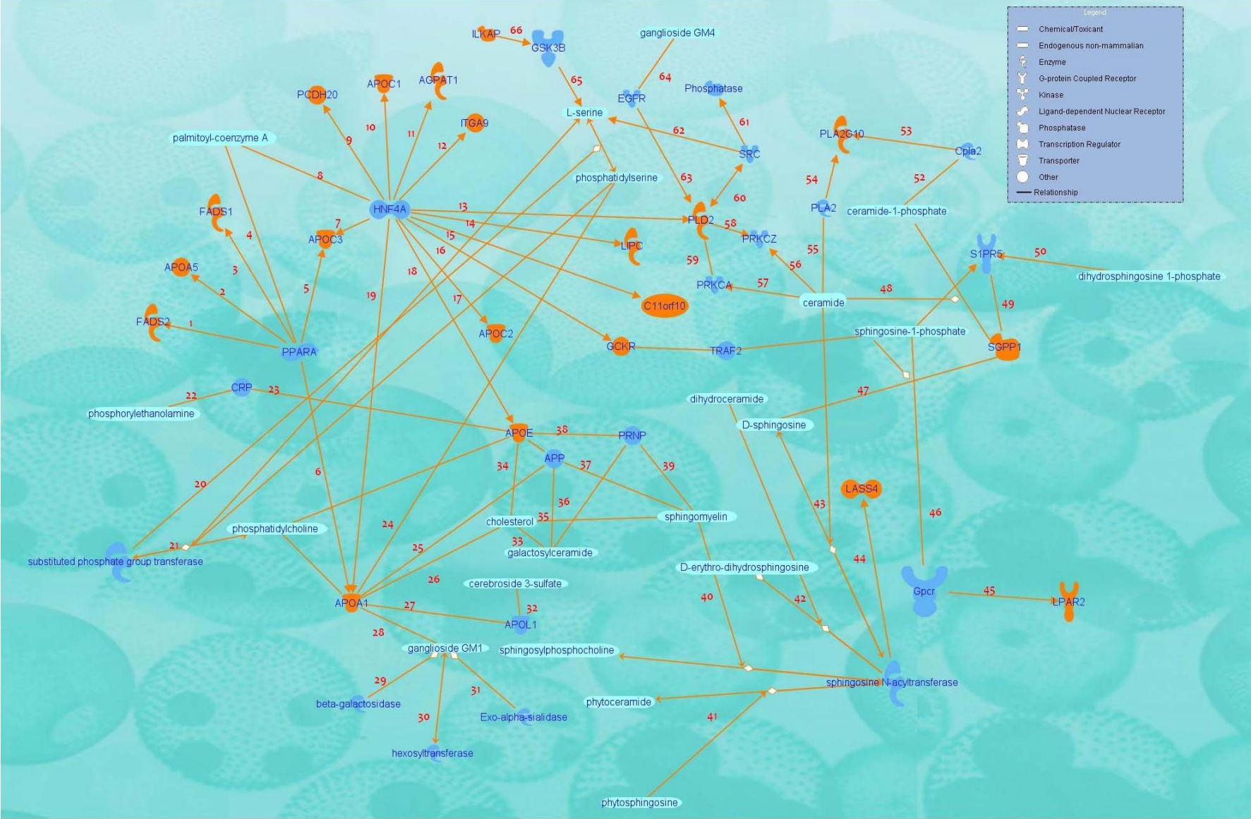
Lipid Pathways by Ingenuity, sphingolipid metabolism.
