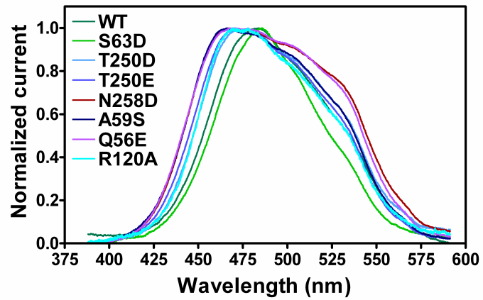
Figure S3: Photoactivation spectra of the ChR2 mutants.
