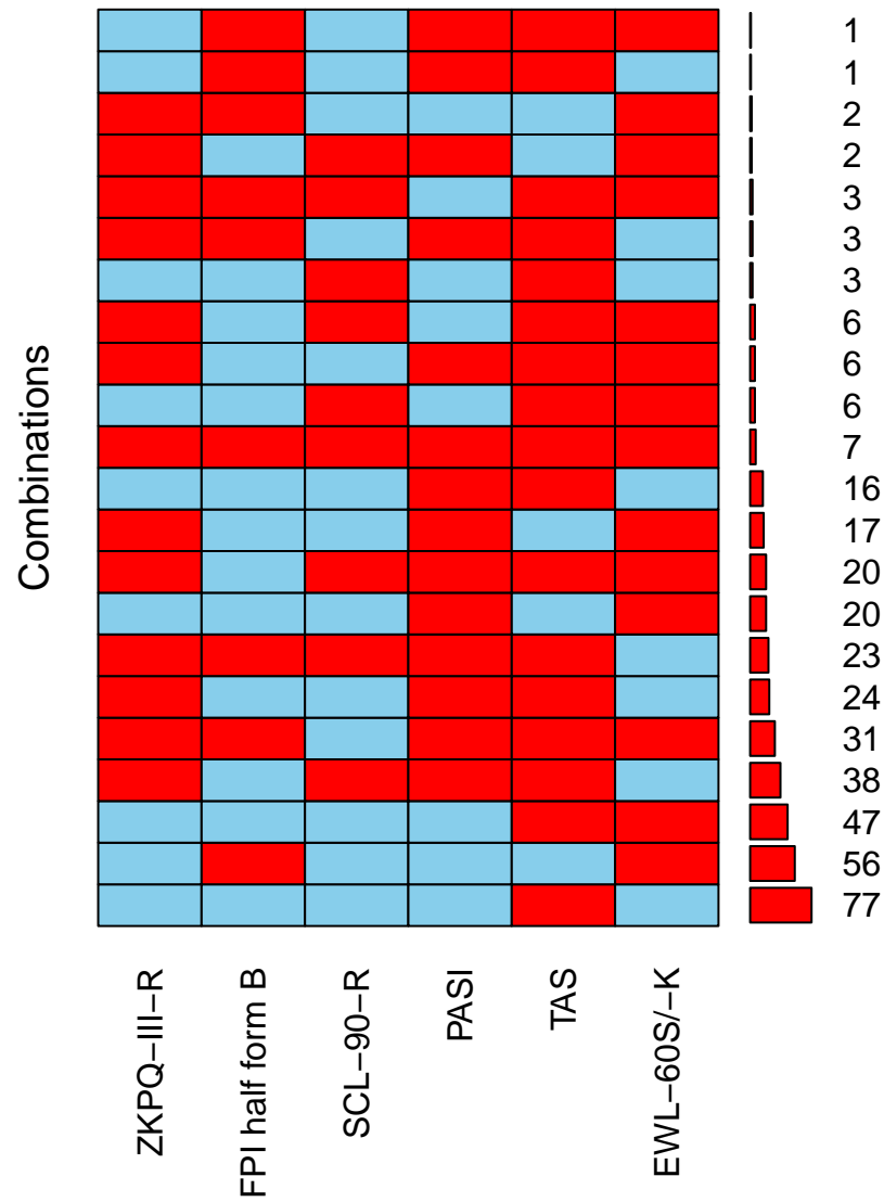
Supplementary Figure 1. Left: Barplot of the proportions of missing values in each questionnaire. Right: All existing combinations of of missing (red) and non-missing (blue) values in the observations.
