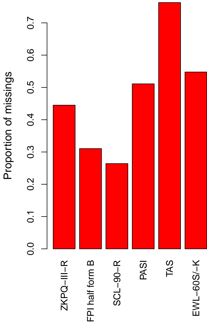
Supplementary Figure 1. Left: Barplot of the proportions of missing values in each questionnaire. Right: All existing combinations of of missing (red) and non-missing (blue) values in the observations.
