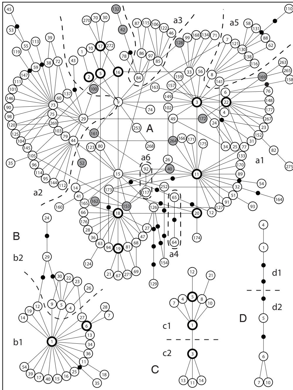
Figure S2: Topology of the MS networks and the sub-haplogroups, with haplotype numbers shown. Haplotypes with grey shade were left unassigned to sub-haplogroups, based on the diagnostic point mutations (Pang et al. 2009). See Figure 3 for more explanations.
