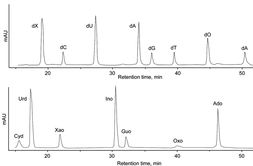
Fig. S1. Resolution of canonical and deaminated ribonucleosides by reversed-phase HPLC. The chromatogram was generated with a mixture of standards, as described in detail in Materials and Methods .
