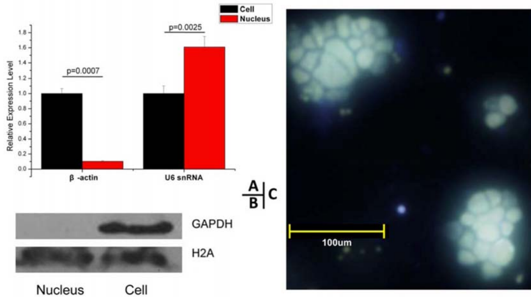
Supplementary information, Figure S1 Assess purity and integrity of nucleus fraction A , Relative enrichment of RNA markers in purified nucleus fraction, equal amount of total RNA was loaded for nucleus and cell extractions. B , Relative enrichment of protein markers in purified nucleus fraction, equal amount of total protein was loaded for nucleus and cell extractions. C Integrity of purified nucleus under fluorescence microscope (Hoechst 33258). Bar, 100 \mu m.
