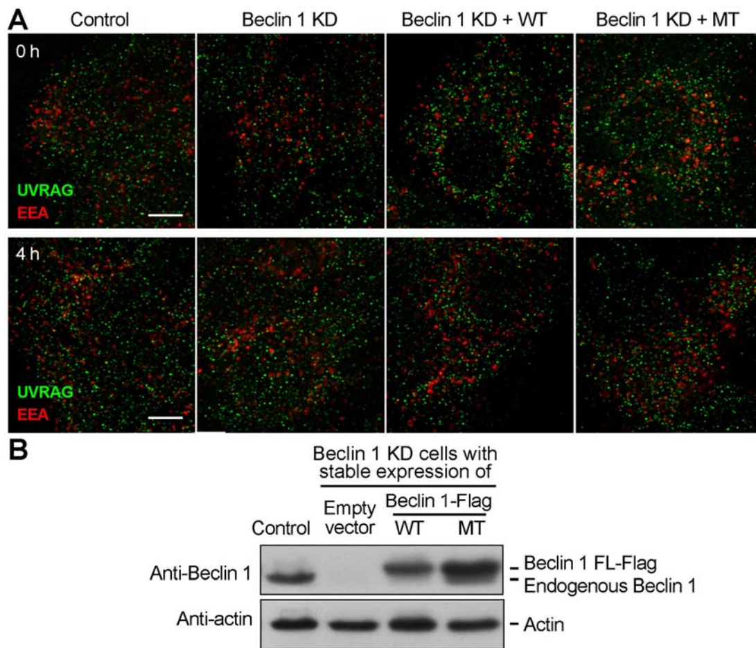
Figure S13 Mutation of the aromatic finger does not alter cellular localization of UVRAG or EEA1 before or after starvation. (A) Shown here are staining patterns for UVRAG (green) and EEA1 (red) in normal HeLa cells (Control), Beclin 1 knockdown HeLa cells (Beclin 1 KD), and Beclin 1 knockdown cells with stable expression of either WT or mutant (MT, F359D/F360D/W361D) Beclin 1. (B) Examination of Beclin 1 expression levels in the four different cells by Western blots.
