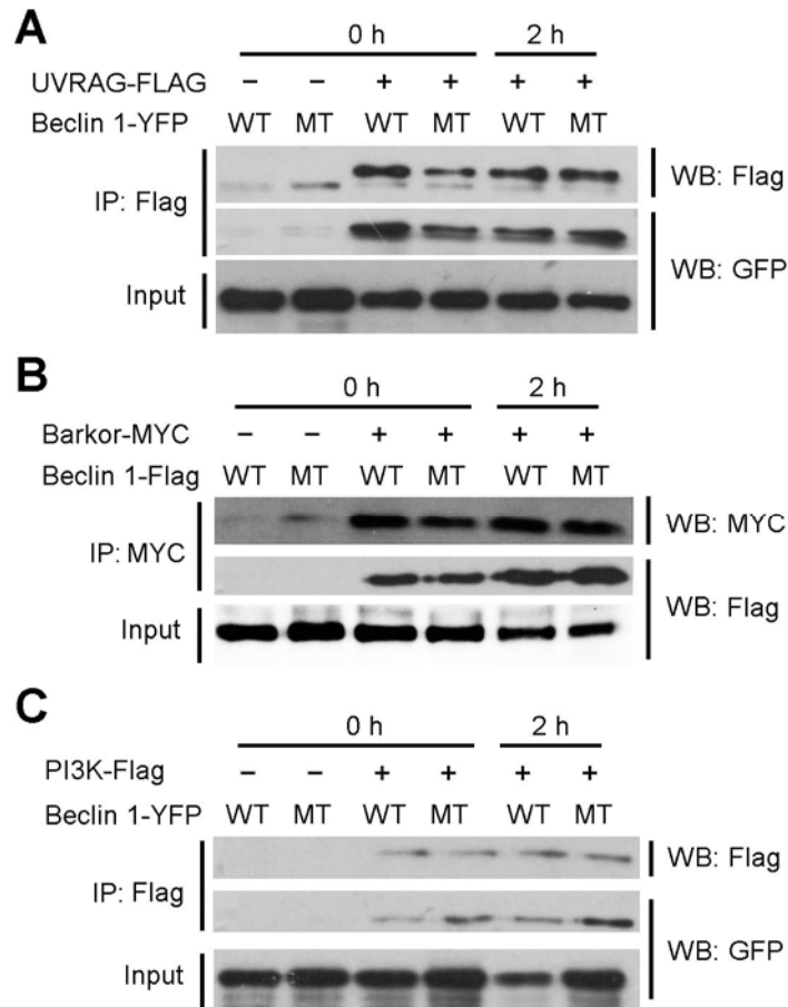
Figure S9 Mutation of the aromatic finger does not affect interactions between Beclin 1 and UVRAG, Barkor, or PI3KC3. (A) The interactions between Beclin 1 and UVRAG were unaffected by mutation of the aromatic finger (F359D/F360D/W361D). Beclin 1-YFP and Flag-UVRAG were co-transfected into 293T cells. UVRAG was immune-precipitated by an anti-Flag antibody; the pellet was subjected to Western blot analysis using anti-Flag or anti-GFP antibodies. WT: wild-type; MT: mutant. (B) The interactions between Beclin 1 and Barkor were unaffected by mutation of the aromatic finger. Experiments in panels B and C were performed similarly as in panel A . (C) The interactions between Beclin 1 and PI3KC3 were unaffected by mutation of the aromatic finger.
