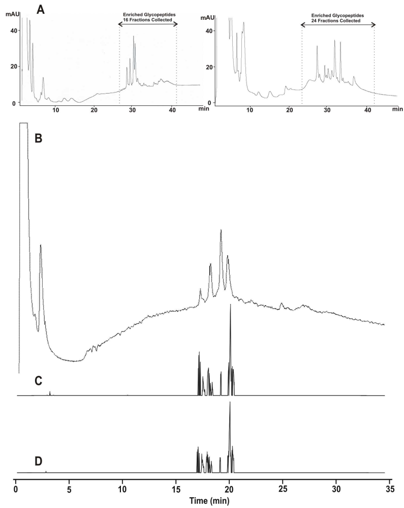
Supplemental figure 1. A) UV traces of tryptic-GluC digest of haptoglobin and tryptic digest of hemopexin separated on a HILIC column. Alignment of the UV trace (chromatogram B) with two extracted ion chromatograms of the data dependent scan of oxonium ions at m/z 204.0 (chromatogram C) corresponding to N-acetylhexosamine and at m/z 366.1 (chromatogram D) corresponding to N-acetylhexosamine-hexose confirm the (glyco)peptide enrichment and separation.
