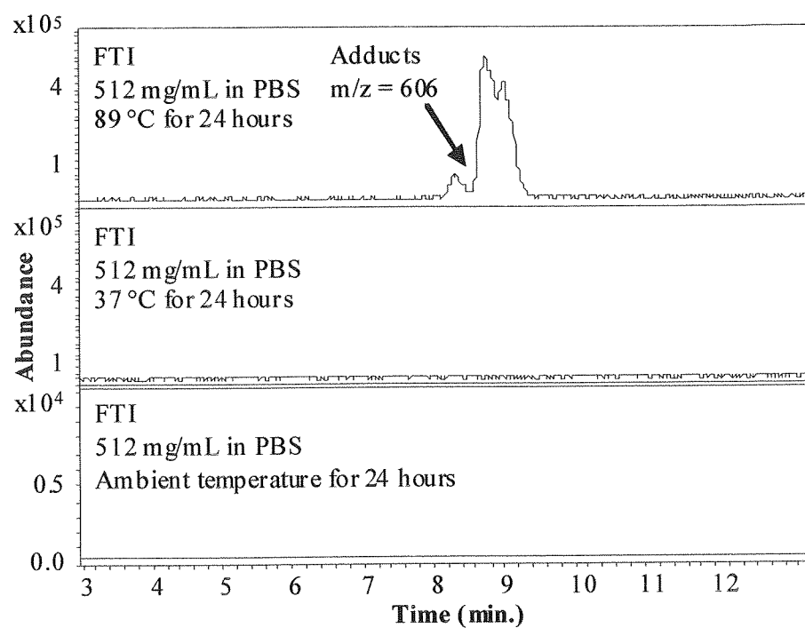
SUPPL. FIG. 2. Extracted ion chromatograms (EIC) of m/z=606 for samples incubated at rt, 37°C and 89°C
