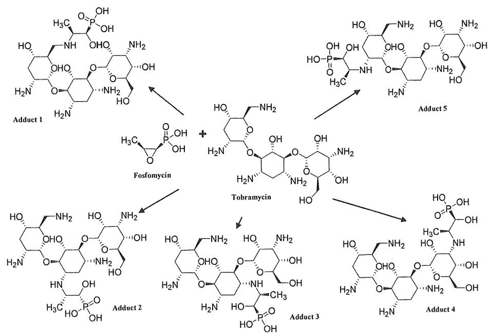
Figure 2. Chemical structures of possible Fosfomicin/Tobramycin adducts
