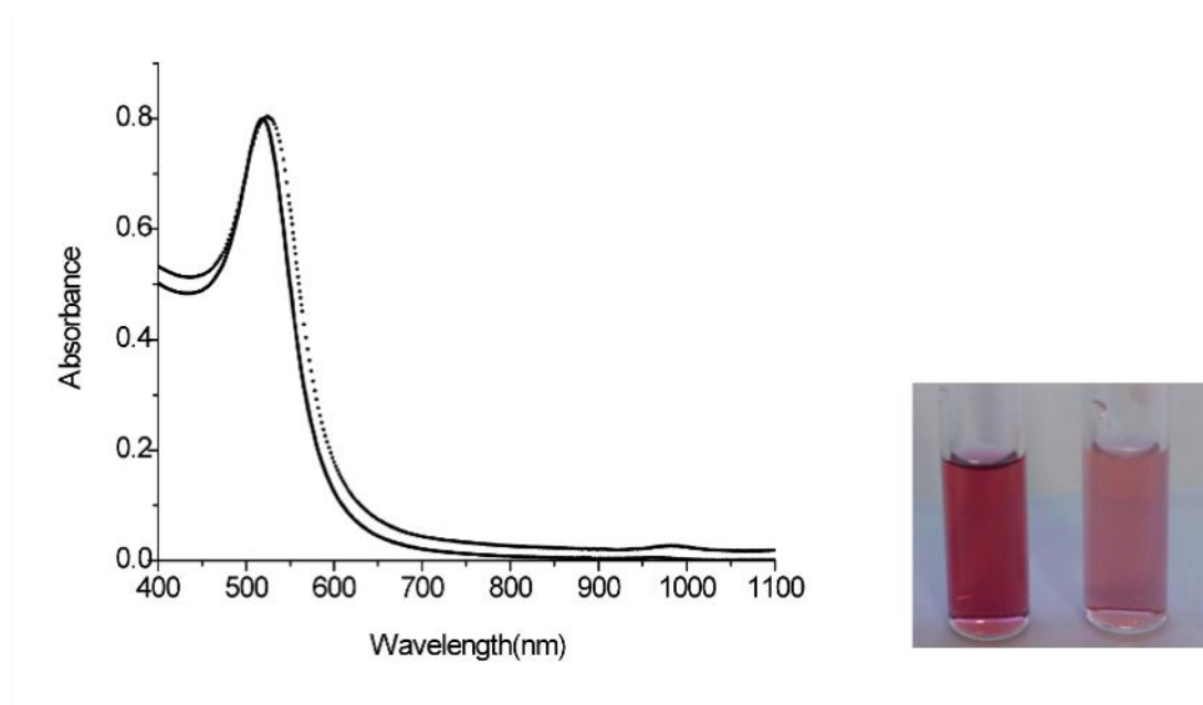
S3. Left) Uv-vis spectra of Citrate-capped gold nanoparticles (solid line) in water and same nanoparticles suspended in DMF (dashed line). Right) Optical photographs of citrate capped nanoparticles in DMF (left) and water (right).
