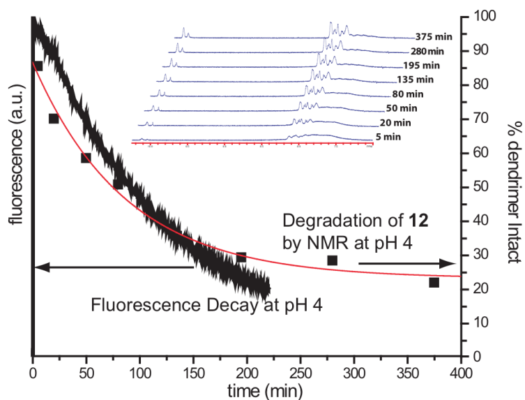
S10. Comparison of fluorescence and NMR degradation at pH 4 in sodium phosphate buffer. Red and black lines represent the degradation determined by NMR and fluorescence, respectively.
