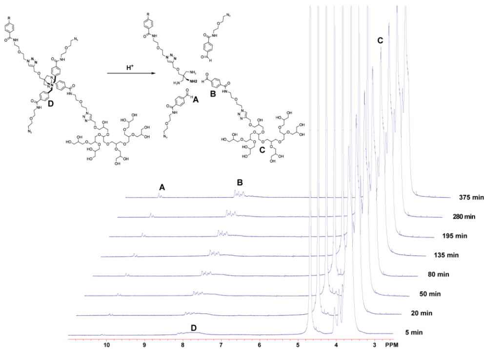
S9. Full NMR spectra of 12 in pH 4 PBS buffer. Showing the formation of aldehyde groups over time upon degradation and the sharpening of the aromatic peaks.
