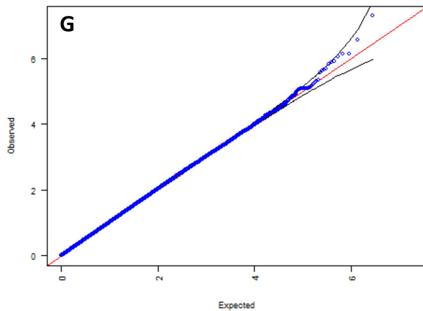
QQ-Plot of PLT ARIC
