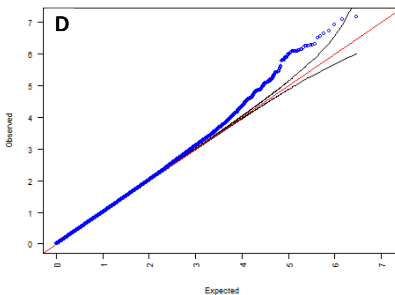
QQ-Plot of PLT Health ABC
