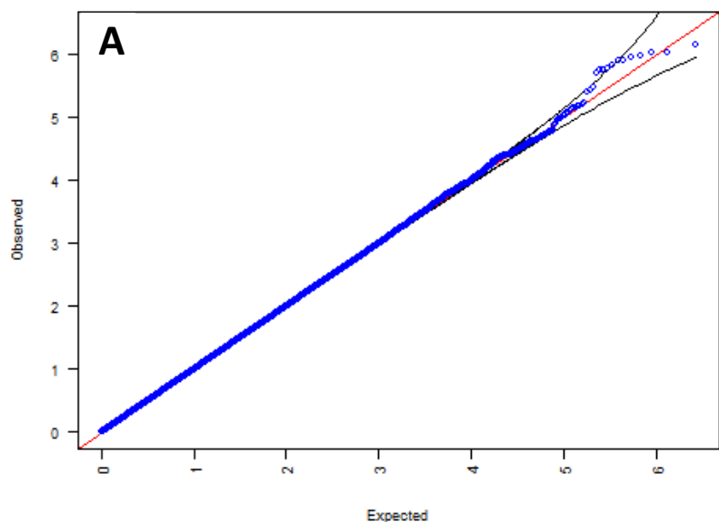
QQ-Plot of PLT WHI
