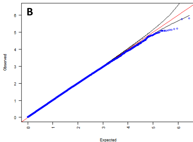
QQ-Plot of PLT Health ABC
