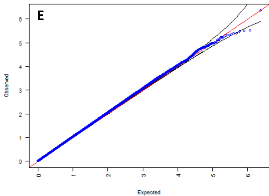
QQ-Plot of PLT GeneSTAR
