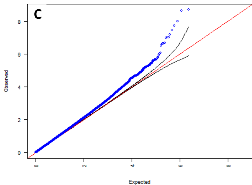
QQ-Plot of PLT WHI
