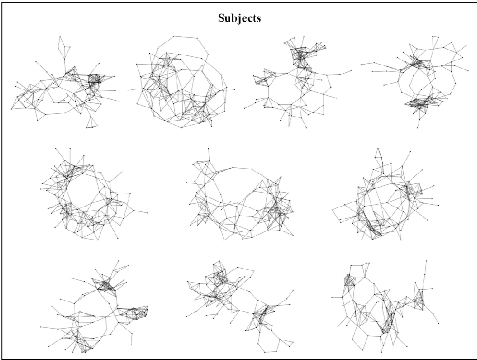
Supplementary Fig. 1. Harel-Koren Fast Multiscale graphs for the 10 subjects' networks.
