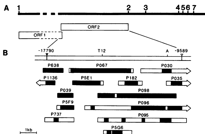
Figure 1. Cloning and sequencing strategy of the ORF1b region of the MHV-A59 polymerase gene. A) The upper line represents the MHV genome. Vertical bars and the numbers above indicate the junction sequences involved in the initiation of the transcription of the corresponding mRNA. Open boxes represent the open reading frames in the polymerase gene. B) The open bar represents the sequenced region of the polymerase gene. The black triangle and the open triangle indicate the start of the large 3'ORF (ORF1b) and the junction sequence for the initiation of mRNA2 transcription, respectively. The positions of oligonucleotides A and T12 are indicated. Negative numbers mark the distance to the start of the poly(A)-tail of the genome. The numbered bars refer to the cDNA clones used for sequencing, the sequenced areas are indicated in black.
