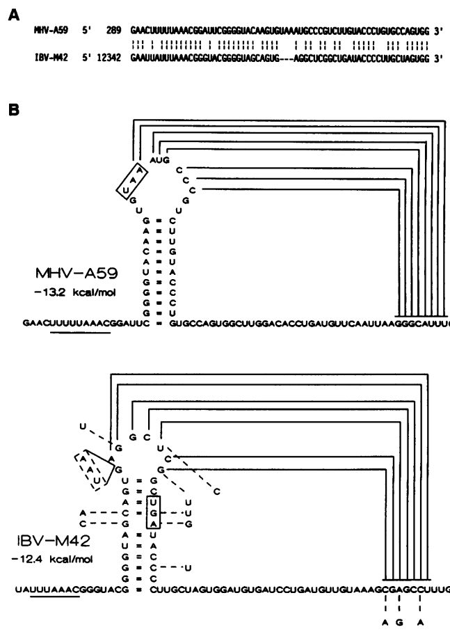
Figure 3. Comparison of the primary and secondary structure of the MHV-A59 and IBV-M42 ORF1a/ORF1b overlap. A) Alignment of the nucleotide sequences. Numbers refer to the position of the 5' G residue in the published sequence (MHV-A59, this article; IBV, ref. 14). B) Predicted secondary and tertiary RNA structure at the site of ribosomal frameshifting. The potential codons involved in frameshifting are underlined, and the termination codons of ORF1a are boxed. Solid lines illustrate the potential pseudoknot. Differences in the nucleotides involved in the predicted RNA structure of MHV in comparison to IBV are indicated in the predicted structure for IBV to illustrate the observed covariation.
