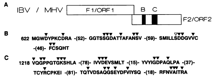
Figure 6. A) Localization of the 'polymerase' (B) and 'helicase' (C) domain in the second ORFs of the IBV and MHV-A59 pol genes. B and C) Amino acid sequence of the conserved domains identified in ORF1b of MHV-A59. Conserved residues are indicated by triangles. Numbers on the left refer to the localization of the conserved domains in the ORF1b sequence. Fig 6B; The 'GDD' or 'polymerase' motif (38, 39). The position of the serine residue which replaces the glycine is indicated with an open triangle. Fig. 6C. The 'GKS/T' or 'helicase' motif (40, 41).
