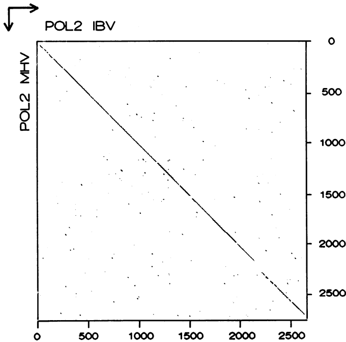
Figure 5. Proportional dot matrix comparison of the amino acid sequences from ORF1b of MHV-A59 and of IBV-M42. Numbers of the amino acid residues are indicated at the axis. For creating the dot-matrix plot the program 'Compare' of the Genetics Computer Group (Wisconsin) (25) was used with a window size of 21 and a stringency of 15.
