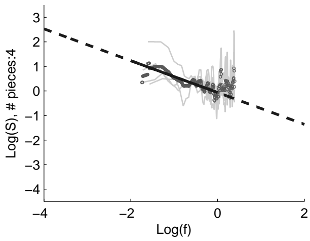
Original spectra
