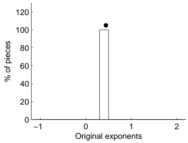
\mu original: 0.440
