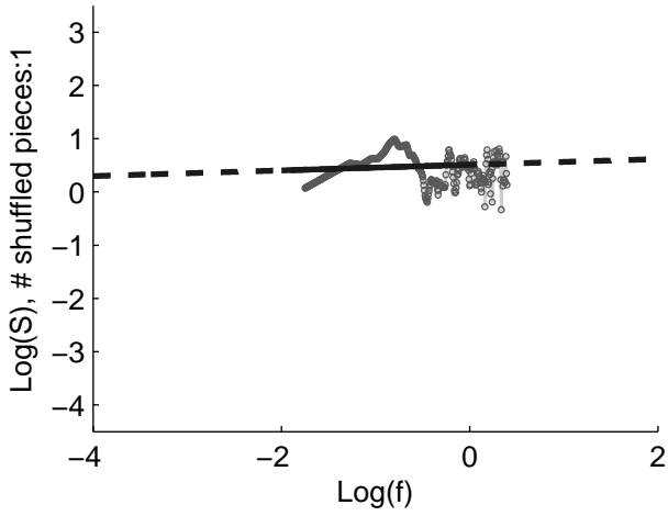
Shuffled spectra
