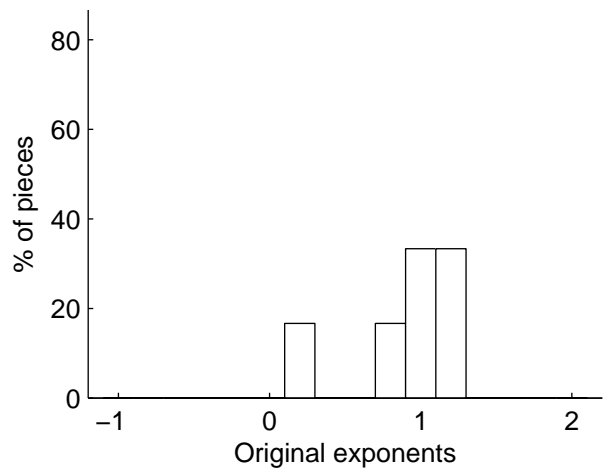
\mu original: 1.013
