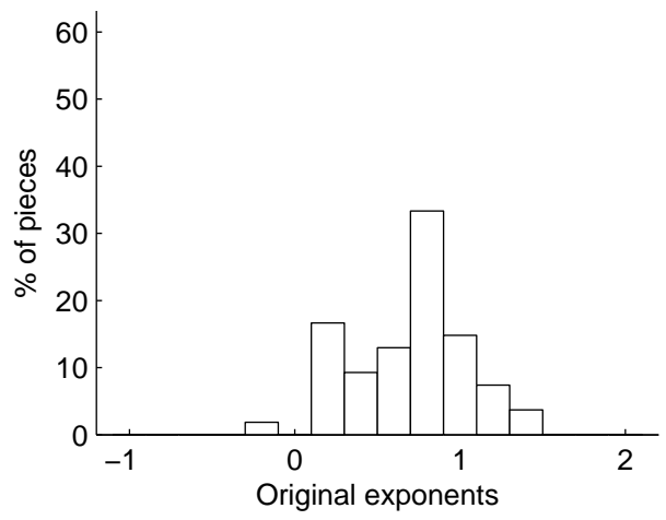
\mu original: 0.735
