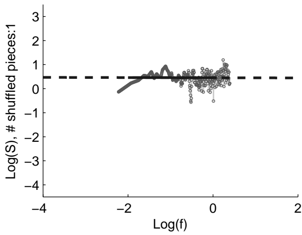
Shuffled spectra
