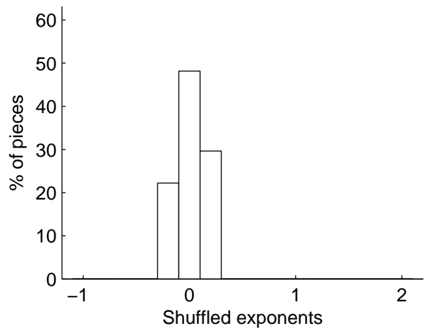
\mu shuffled: 0.030
