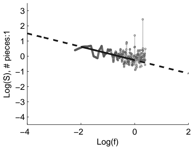
Original spectra
