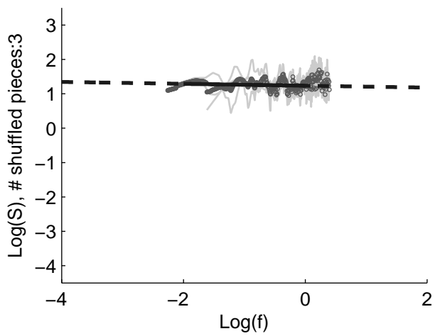
Shuffled spectra
