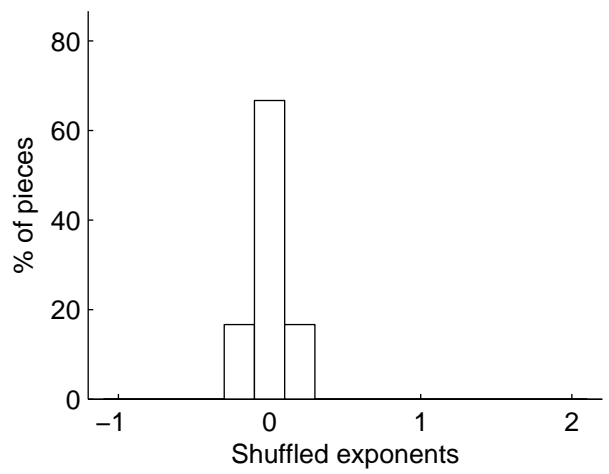
\mu shuffled: 0.049
