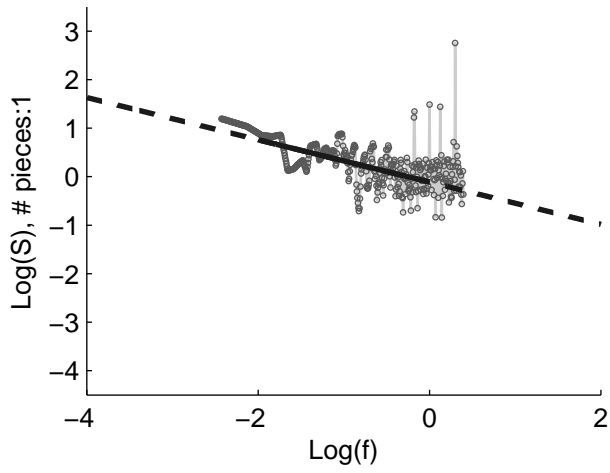
Original spectra
