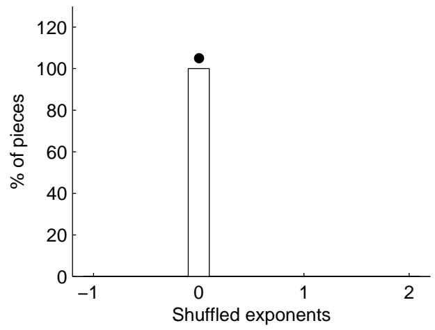
\mu shuffled: 0.004
