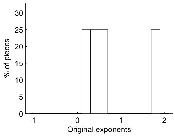
\mu original: 0.561
