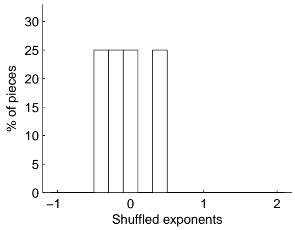
\mu shuffled: -0.132
