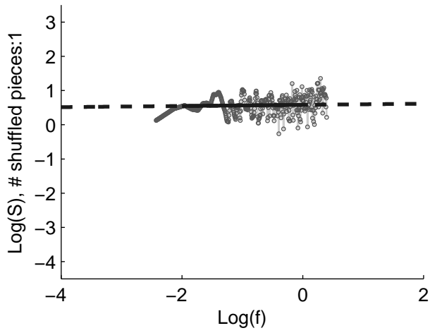
Shuffled spectra
