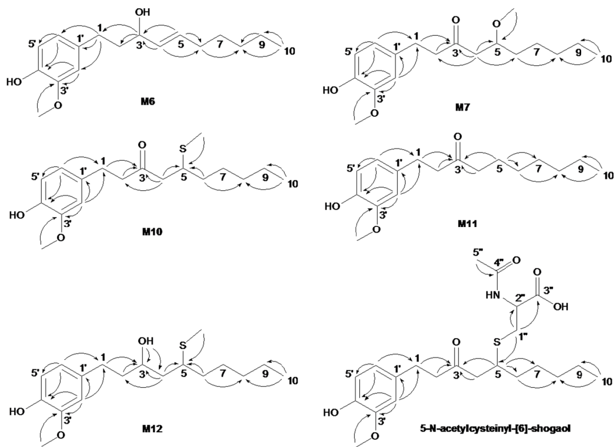
Supplementary Figure 1. Key HMBC correlations of M6, M7, M10–M12 and synthetic 5-N-acetylcysteinyl-[6]-shogaol.
