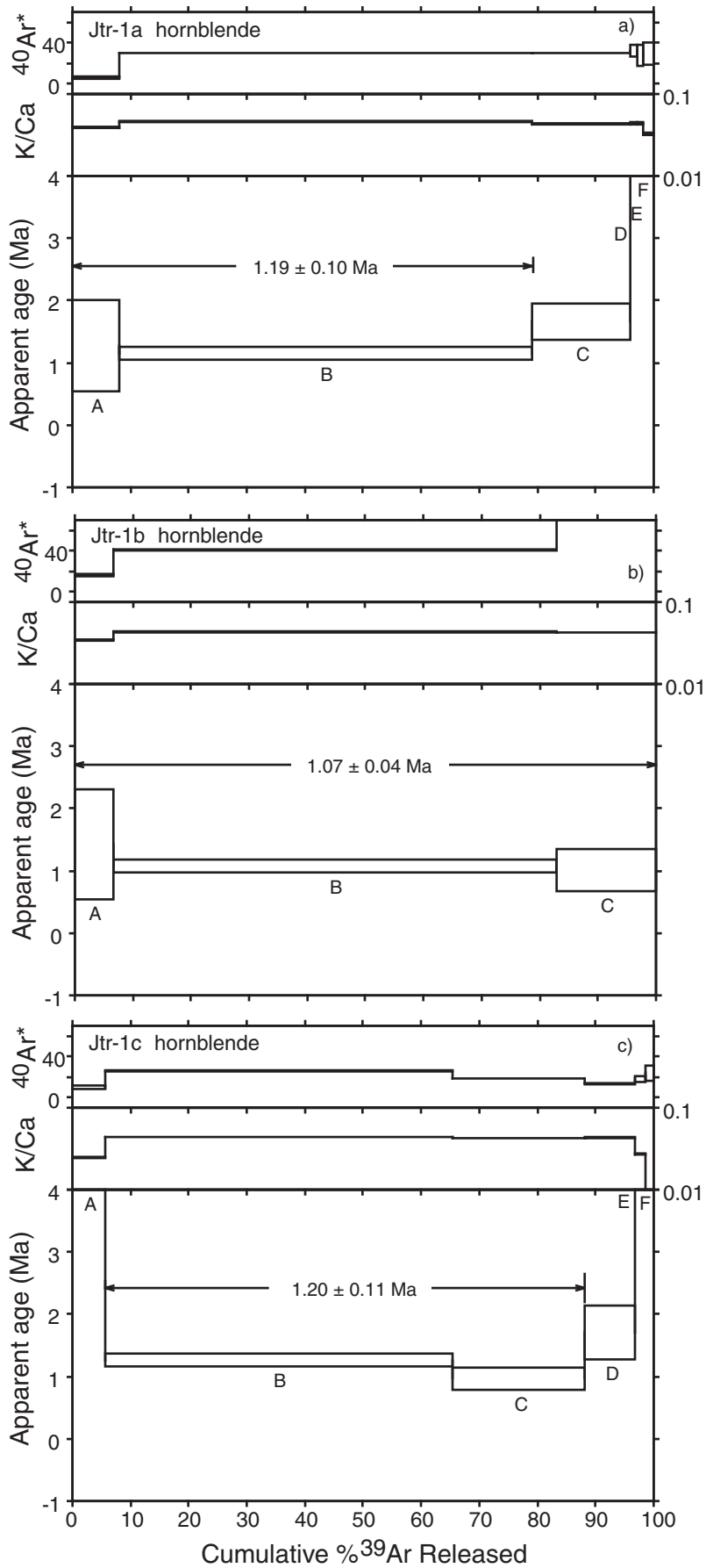
Fig. 5. Age spectra, K/Ca, and radiogenic yield diagrams for step-heating results of hornblende sample Jtr-1.
