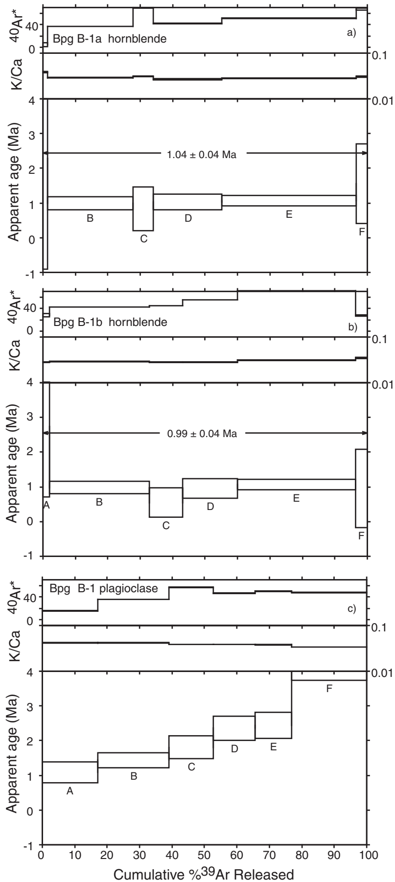
Fig. 6. Age spectra, K/Ca, and radiogenic yield diagrams for step-heating results of sample Bpg B-1 hornblende (a and b) and plagioclase (c).
