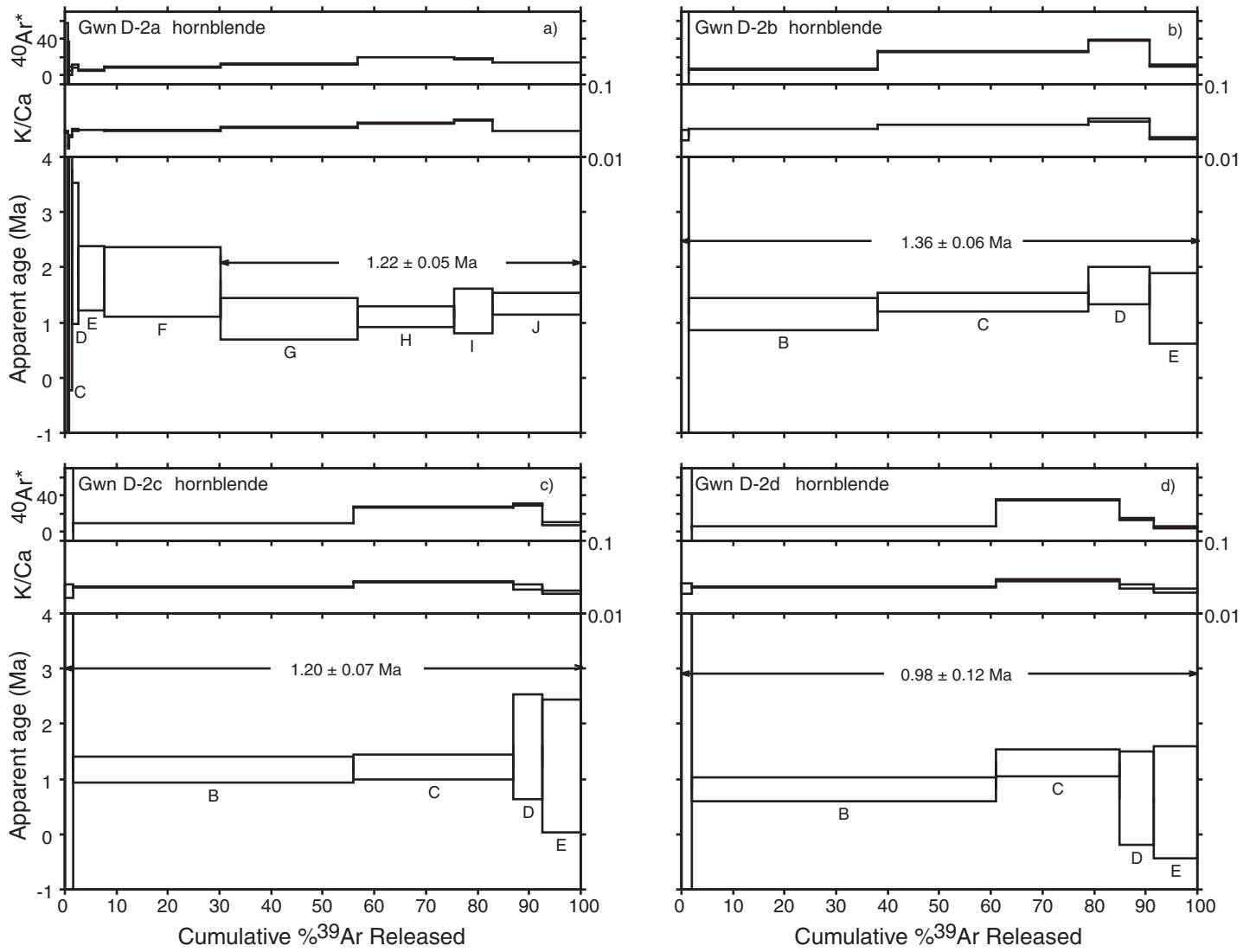
Fig. 7. Age spectra, K/Ca, and radiogenic yield diagrams for step-heating results of hornblende sample Gwn D-2.
