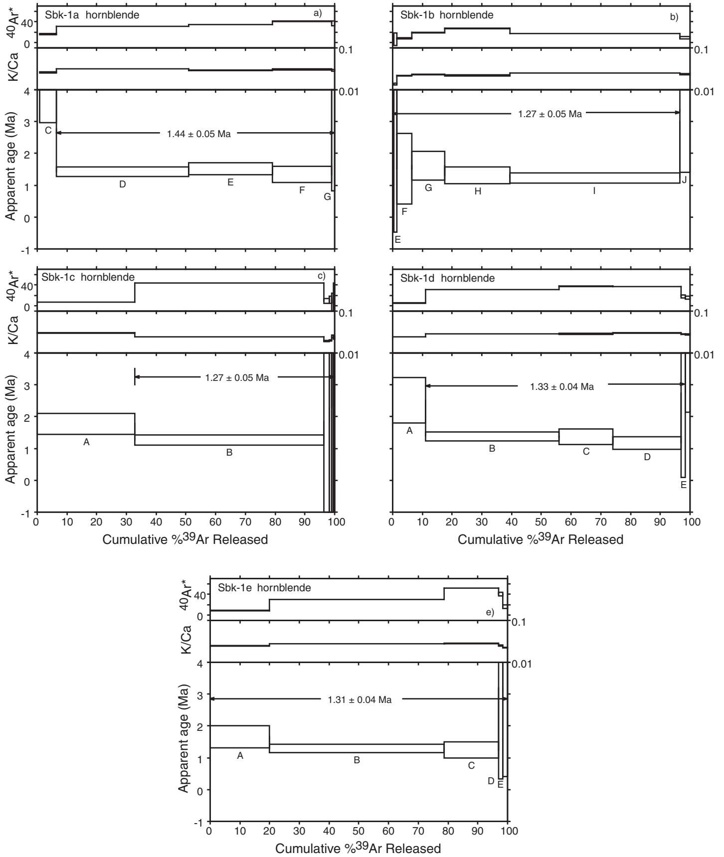
Fig. 8. Age spectra, K/Ca, and radiogenic yield diagrams for step-heating results of hornblende sample Sbk-1.
