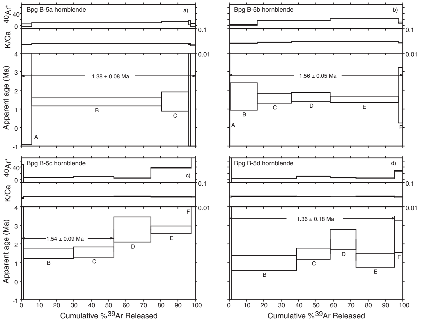
Fig. 11. Age spectra, K/Ca, and radiogenic yield diagrams for step-heating results of hornblende sample Bpg B-5.
