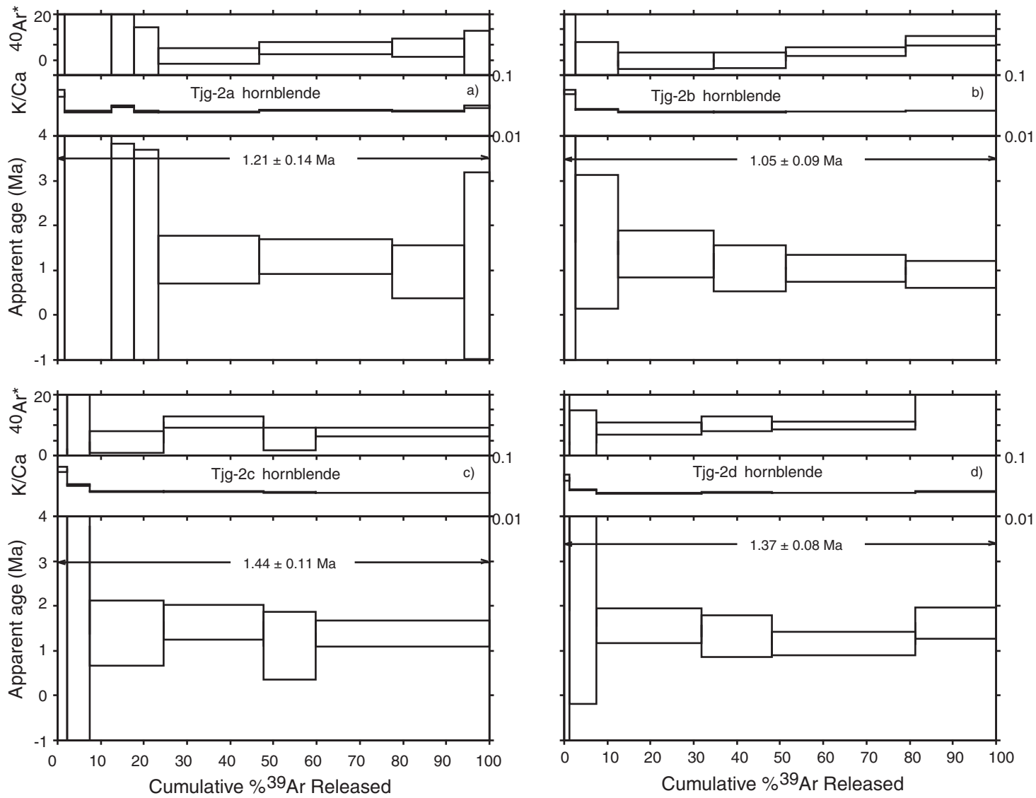
Fig. 13. Age spectra, K/Ca, and radiogenic yield diagrams for step-heating results of hornblende sample Tjg-2.
