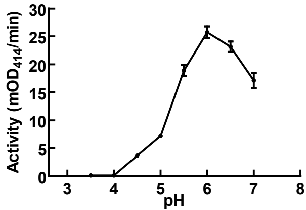
ABTS
