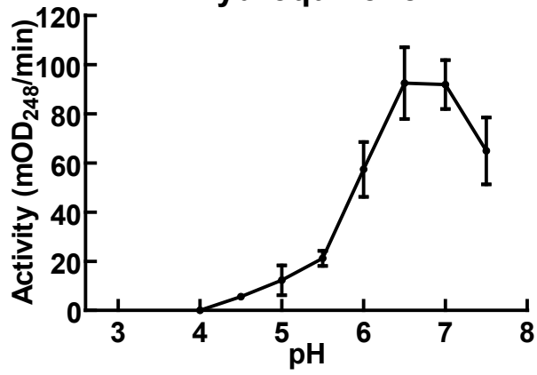
Hydroquinone
