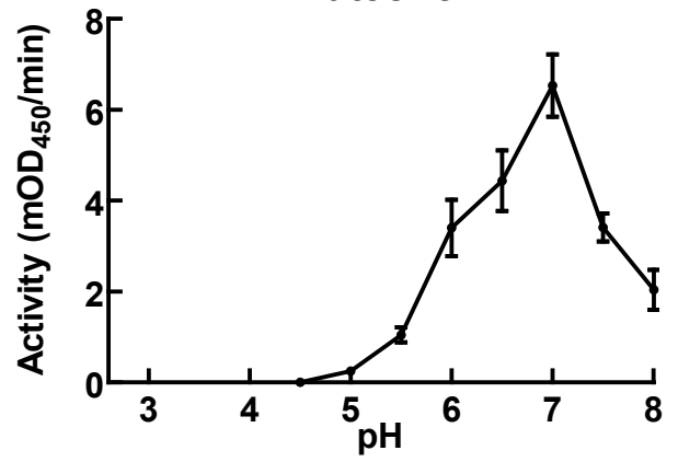
Catechol
