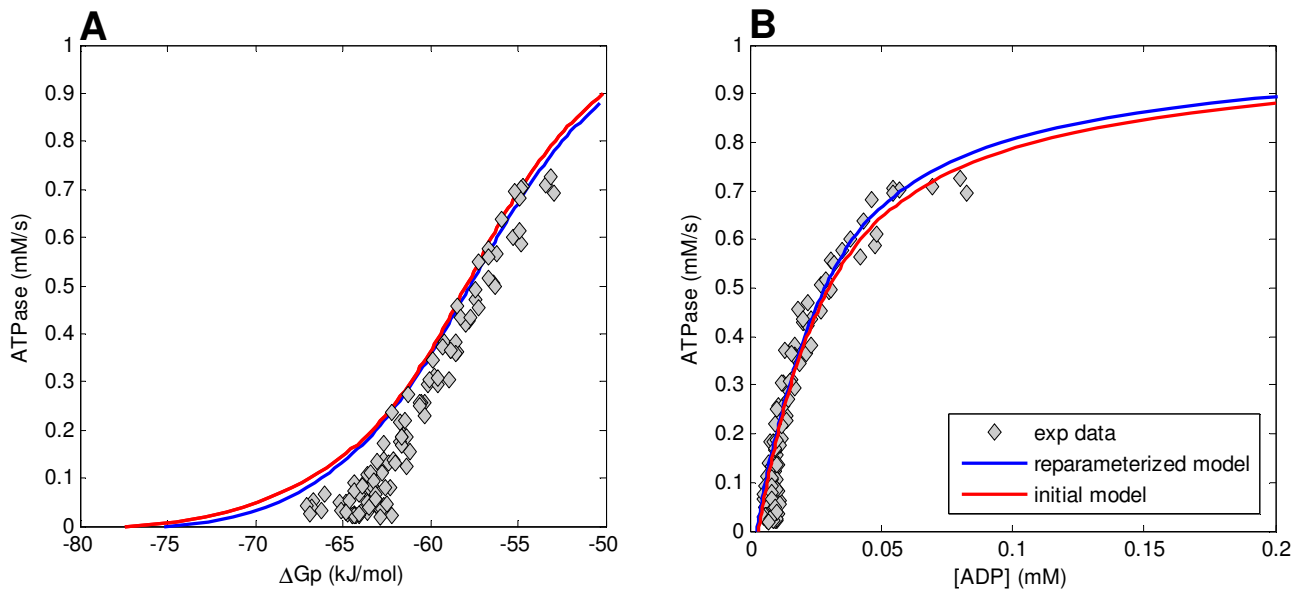
Figure 3 , predictions according to the initial model (red lines; the same result as the red line in Figure 1 in the main text) and reparameterized model (blue lines) compared to experimental data (grey diamonds) sampling the \Delta G_p - J_p (A) and ADP - J_p relation (B). The reparameterized model was obtained by including both the \Delta G_p - J_p and ADP - J_p data in the parameter estimation procedure. The transduction function of the reparameterized model became very similar to the initial model and was rejected because it failed to describe rest and low exercise conditions.
