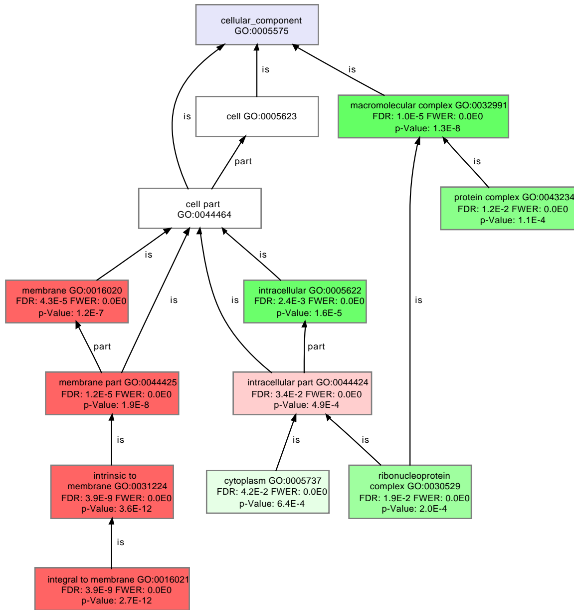
Enriched Graph
