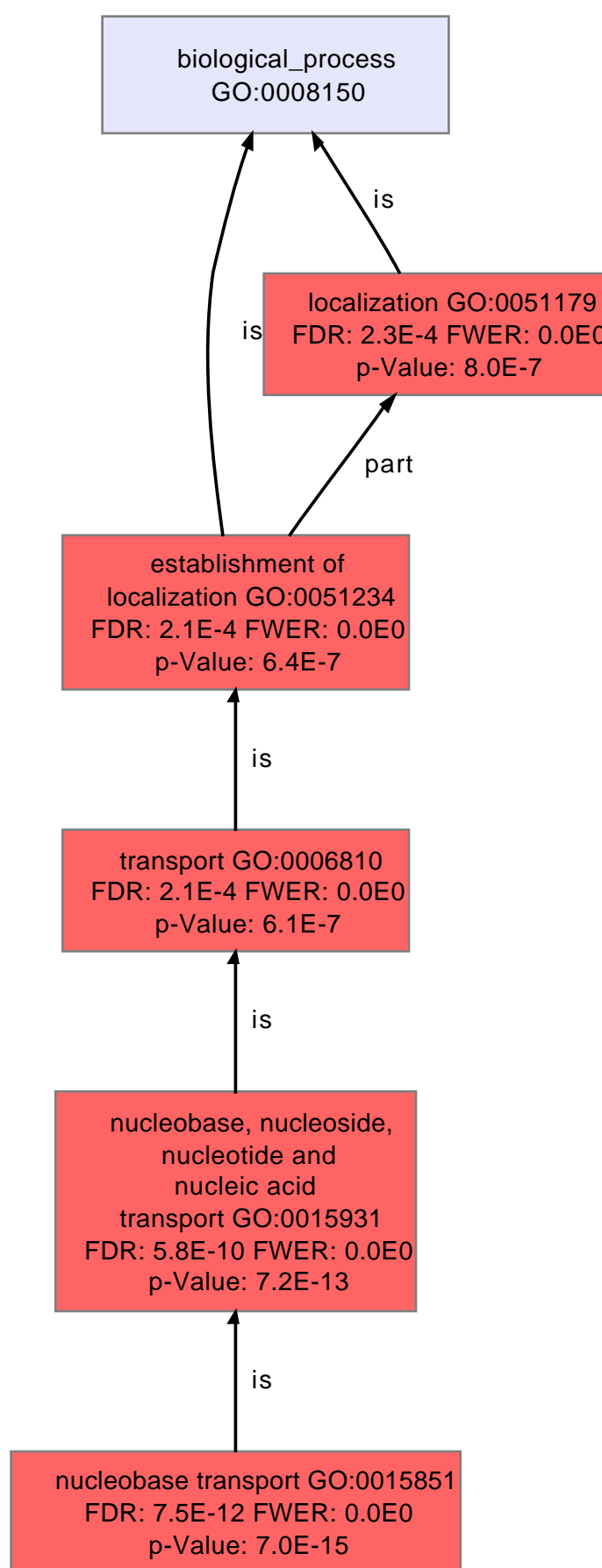
Enriched Graph
