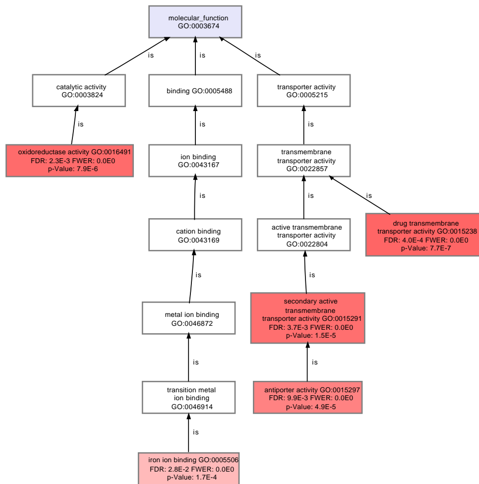
Enriched Graph
