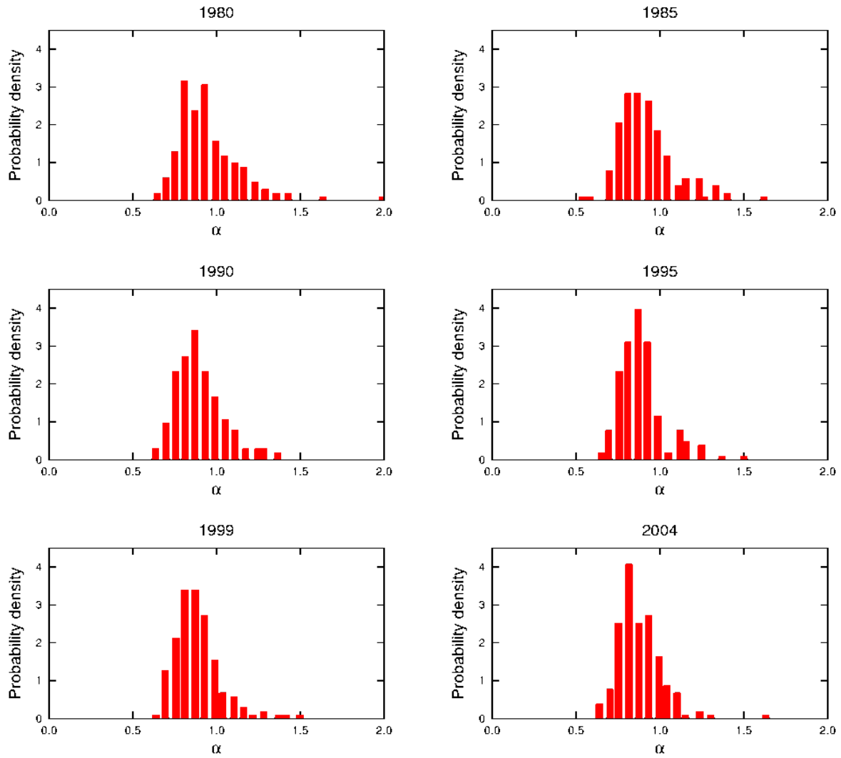
Figure S116: Probability density distribution of the transformation exponent \alpha for various publication years.
