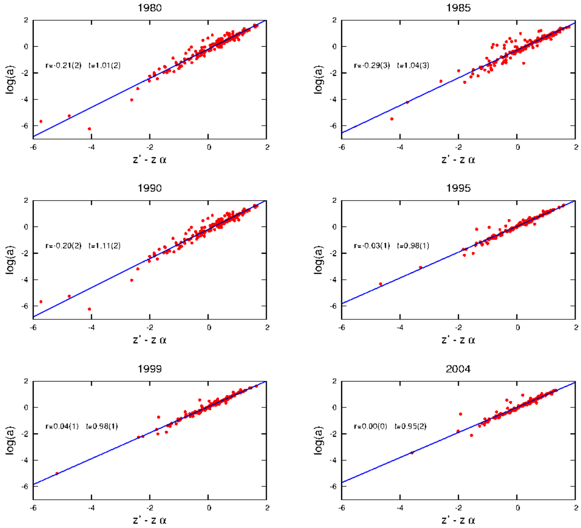
Figure S115: \log(a) = r + t(z' - z\alpha) .
