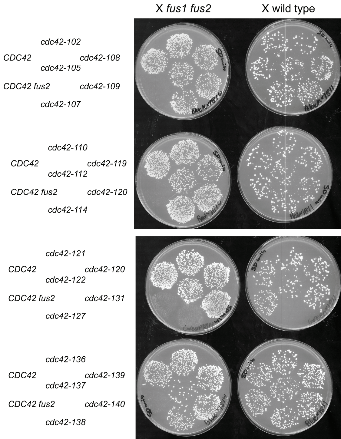
Supplementary Figure 1 Screen of Cdc42 alanine-scanning alleles with cell fusion defects
