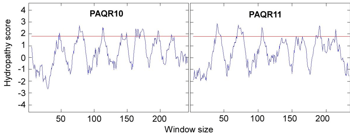
Figure S1 Hydrophobicity analysis of PAQR10 and PAQR11.
