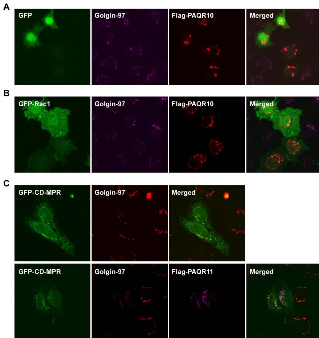
Figure S6 Control experiments for confocal studies. (A) PAQR10 does not colocalize with GFP. HeLa cells were transfected with GFP and Flag-tagged PAQR10, following by immunostaining and confocal analysis. (B) PAQR10 does not colocalize with Rac1. HeLa cells were transfected with GFP-fused Rac1 and Flag-tagged PAQR10, following by immunostaining and confocal analysis. (C) PAQR11 cannot increase the localization of CD-MPR in the Golgi apparatus. HeLa cells were transfected with GFP-fused CD-MPR with or without Flag-tagged PAQR11, following by immunostaining and confocal analysis.
